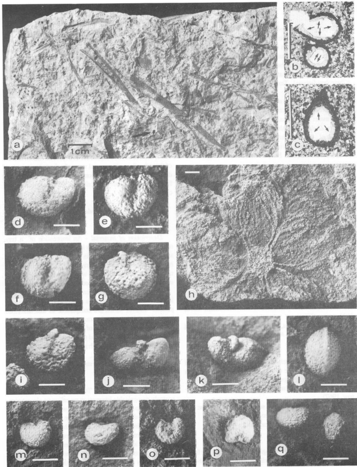
Figure 4: Plant macrofossils from the Gross Brukkaros lake beds, Namibia. Unless otherwise stated scale bars are 1 mm. a) Assemblage of plant litter with fragments of axes in subparallel preferred orientation and pits caused by former carpoliths, GB 91 7a. Arrow indicates carpolith impression that is shown as replica in j; b-c) Photomicrographs of thin sections showing transverse sections of Carpolithus B. Black = oxidised goethite, little arrows indicate boundary of calcite wallpaper; b = GB 91 7d, c = GB 91 7a; d) Carpolithus A, latex cast, GB 91 S2a; e) Carpolithus A, latex cast, GB 91 S1b; f) Carpolithus A, latex cast, GB 91 7a4II; g) Carpolithus A, latex cast, GB 91 7a3III; h) ?angiospermous flower, latex cast, GB 91 S1; i) Carpolithus A, latex cast, GB 91 7aIII; j) Carpolithus A, latex cast, GB 91 7a1; k) Carpolithus A, latex cast, GB 91 S1a; l) Carpolithus B, latex cast, GB 91 7fa; m) Carpolithus C, latex cast, GB 91 S2b; n) Carpolithus C, latex cast, GB 91 7aIII; o) Carpolithus C, latex cast, GB 91 Sib; p) Carpolithus C, latex cast, GB 91 S2a; q) Carpolithus C, latex cast, GB 91 7fb
