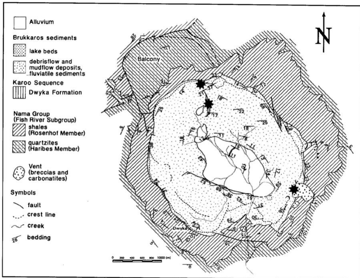
Figure 2: Geological map of Gross Brukkaros (modified from Stachel et al. , 1993). Stars indicate sample locations
