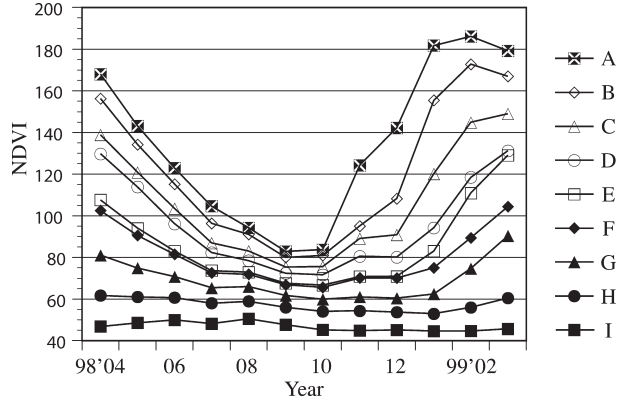
Fig. 2. Monthly changes of mean VGT-NDVI of the classes.
