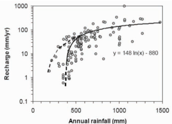
Figure 5.14: The relation between rainfall and groundwater recharge for Southern Africa. Source: Cave et al. (2003)
