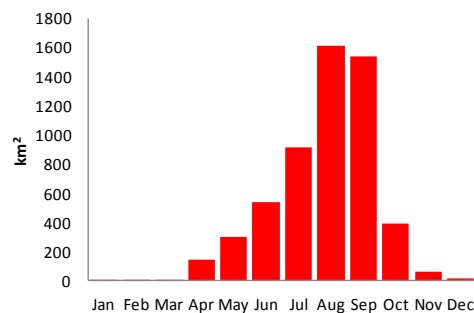
Long term mean (LTM)
