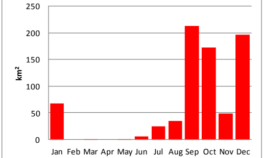
Long term mean (LTM)
