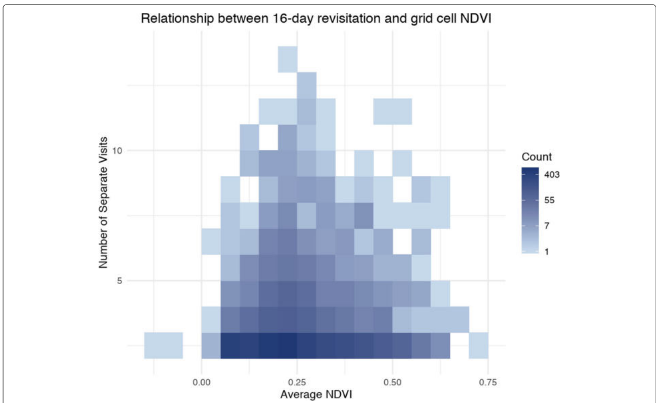
Fig. 7 Relationship between 16-day revisitation and grid cell NDVI. A heat map showing the density of points along axes of number of separate points and mean NDVI values. The color scale is log transformed to better visualize the variability at the lower end of the nsv measure. Note that the highest density of grid cells have 2 visits and a mean NDVI of \approx 0.25 . This plot does not include grid cells not visited or returned to, i.e. nsv < 2
