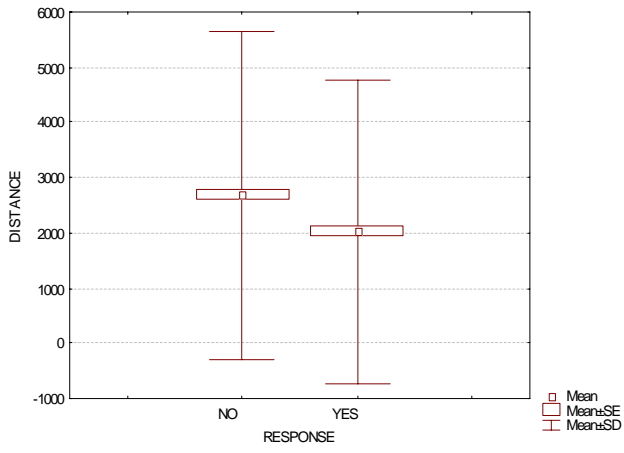
Distance to rivers (Ns)
