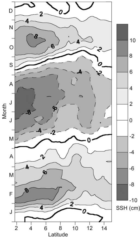
Fig. 6. The propagation of sea surface height anomalies southwards through Angola, indicating the influence of internal waves from the equatorial Atlantic on events in Angola, rather than upwelling wind stress, which declines and orientates onshore as latitude decreases. Only off Peru, where the Andes separate low level winds from the inter-tropical convergence zone in the Amazon basin, do alongshore winds persist to low latitudes.
