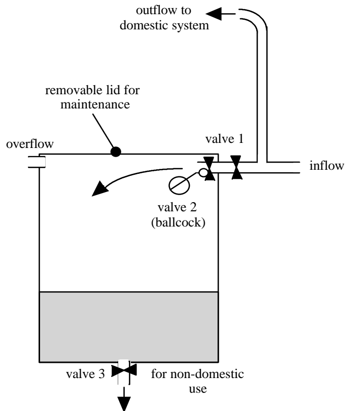
Figure 4-3 Alternative Rinsewater Tank
