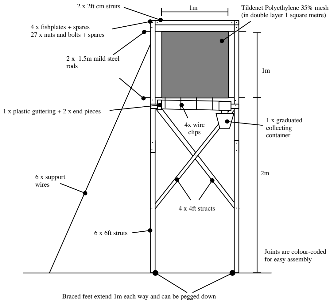
Figure 10-1 Example SFC design
