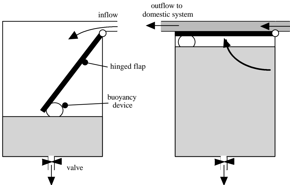
Figure 4-2 Rinsewater Tank Design
