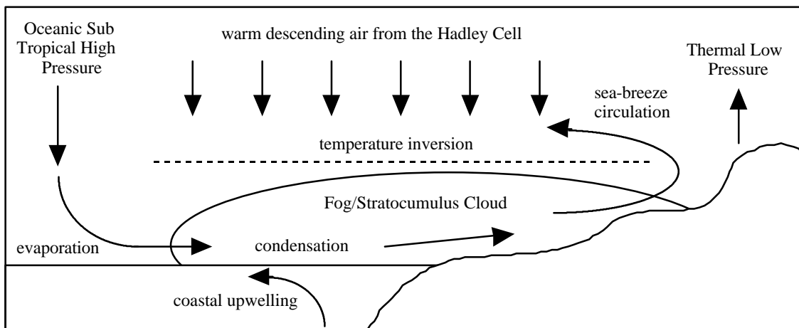
Figure 2-2 West Coast Advection Fog
