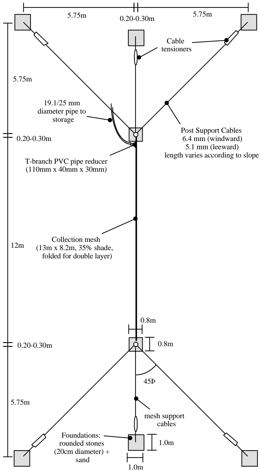
Figure 10-4 48m 2 FCU (Plan View)
