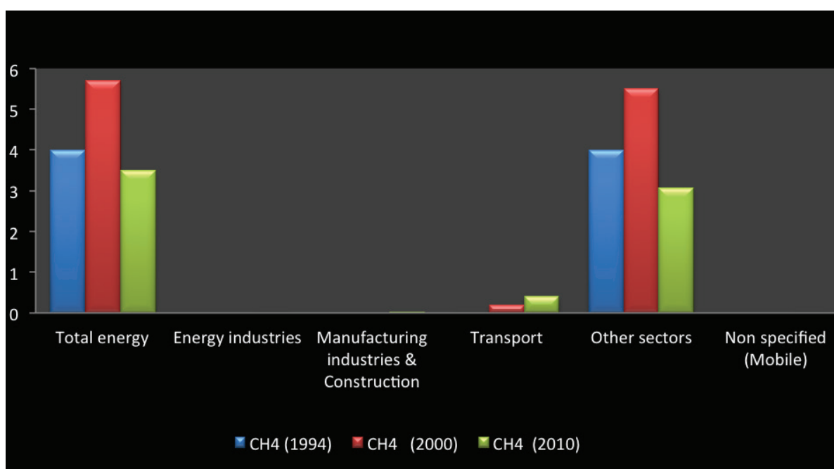
Figure 2.7. CH 4 emissions (Gg) from different categories for 1994, 2000 and 2010
