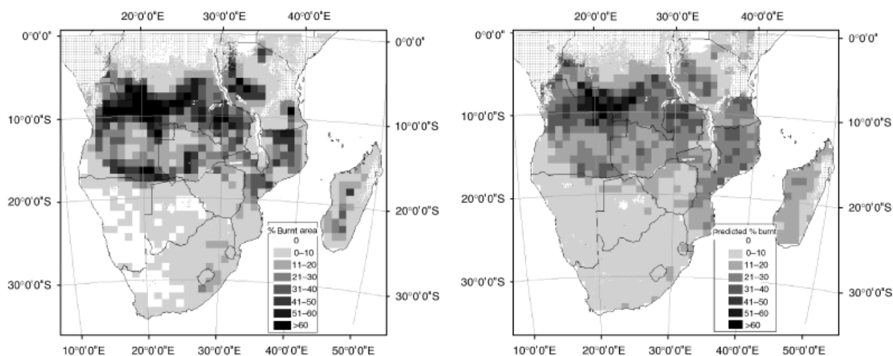
Fig. 5 Observed (left) and predicted (right) percent burnt areas for 100 km × 100 km windows across southern Africa. Predictions are mean values for the reserve samples in the random forest (see 'Data and methods'). Dark stipples represent areas where cloud or missing Moderate Spatial Resolution Spectroradiometer (MODIS) data preclude burned area mapping for more than 5 months of the year.
