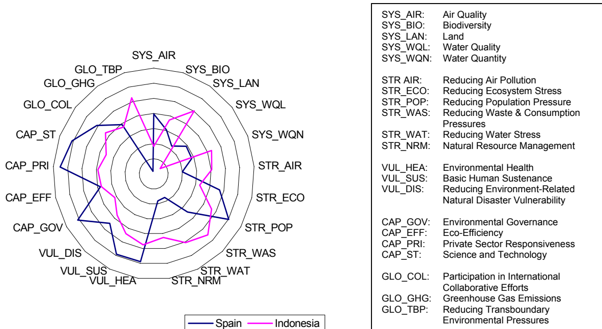
Figure 2: Comparison of Indicator Scores for Spain and Indonesia
