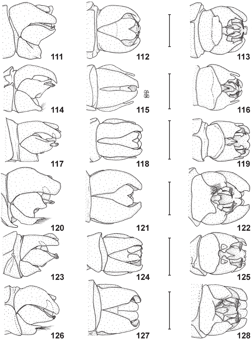
Figs 111–128. Male terminalia of Anclorhynchus species in lateral, dorsal and ventral views: (111–113) A. prunus Oldroyd 1974, holotype; (114–116) A. reynaudii (Macquart, 1838), holotype quadrimaculatus ; (117–119) A. similis sp. n., holotype; (120–122) A. simpsoni sp. n., holotype; (123–125) A. snowi sp. n., holotype; (126–128) A. sokokensis sp. n., holotype. Scale lines = 1 mm.
