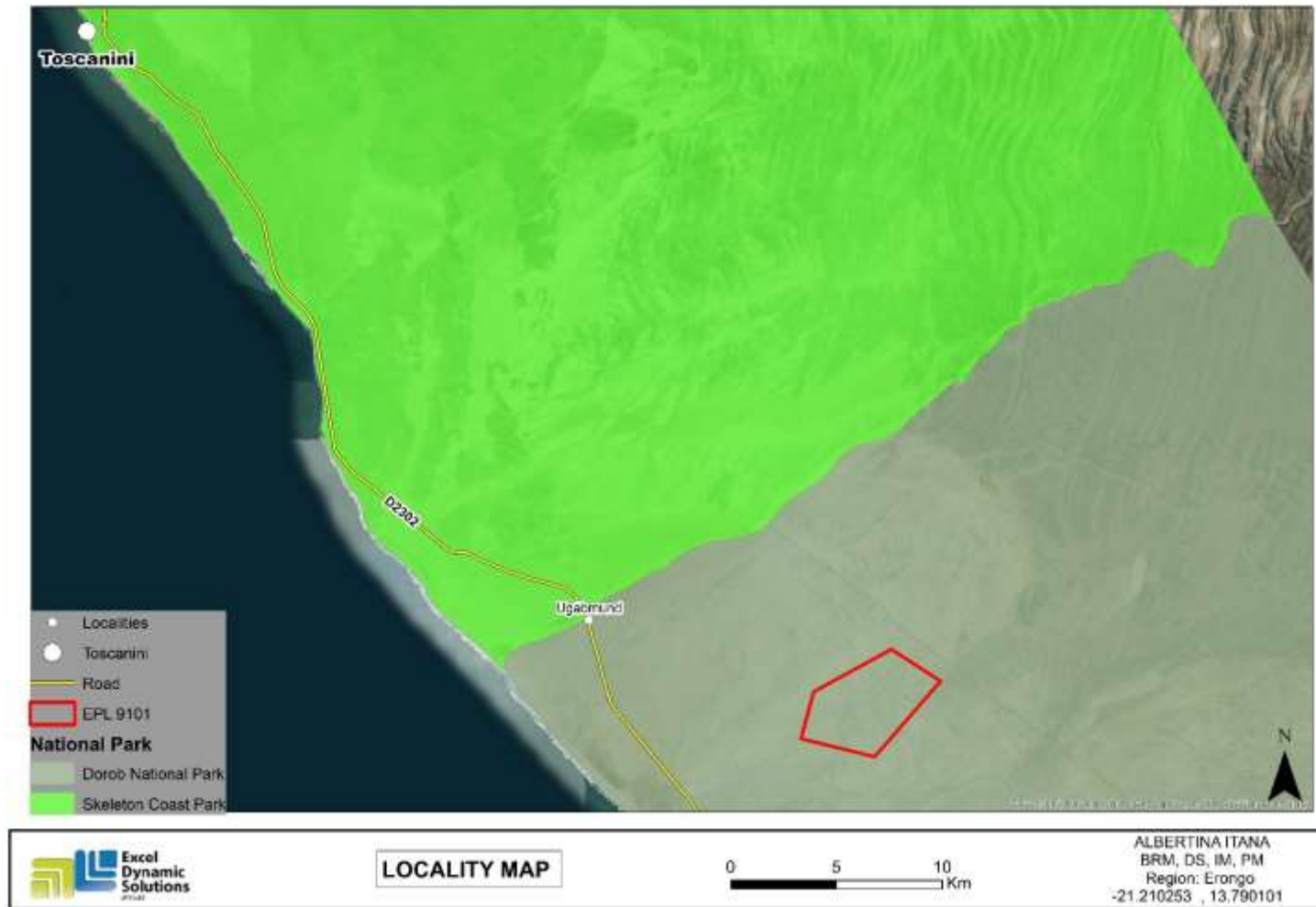
Figure 1: Locality map of EPL 9101 located near Uis.
