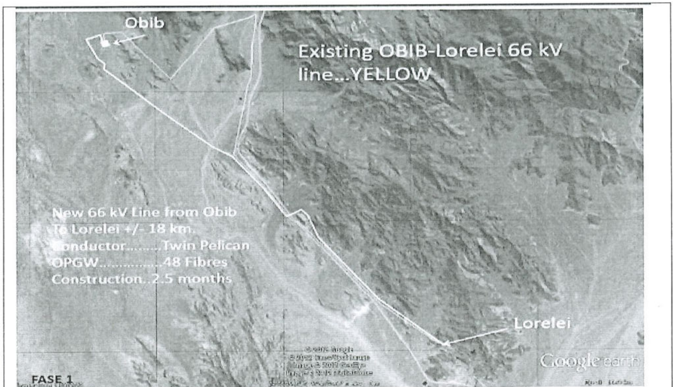
Alignment of proposed new 66 kV power line from Obib to Lorelei substation.
