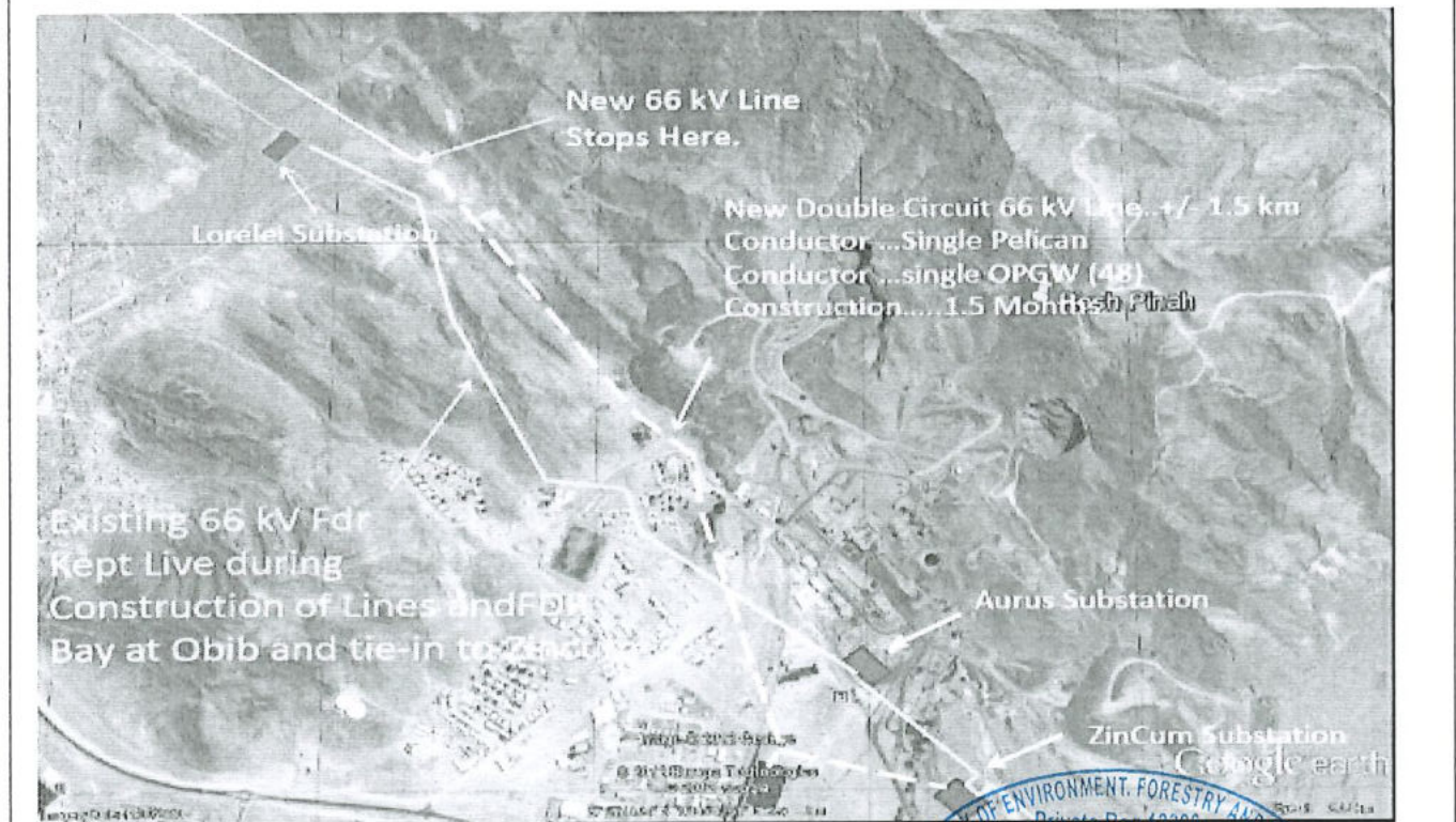
Alignment of the proposed 66 kV power line from Lorelei to Zincum substation.
