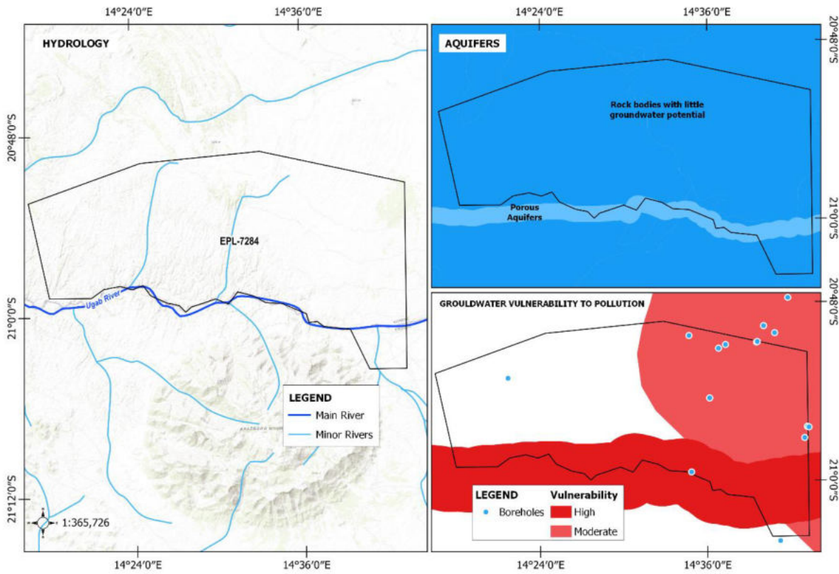
Figure 7: Hydrology and groundwater vulnerability map
