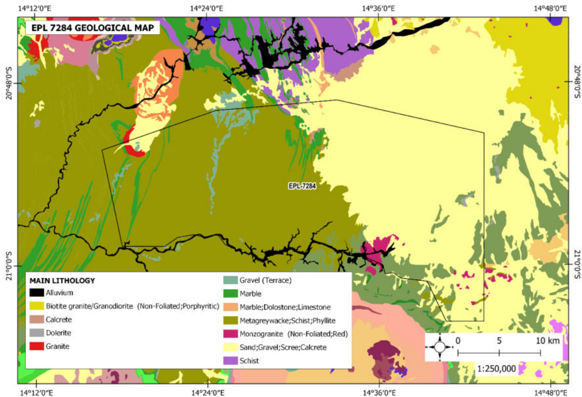
Figure 4: A map of the general geology of the project area
