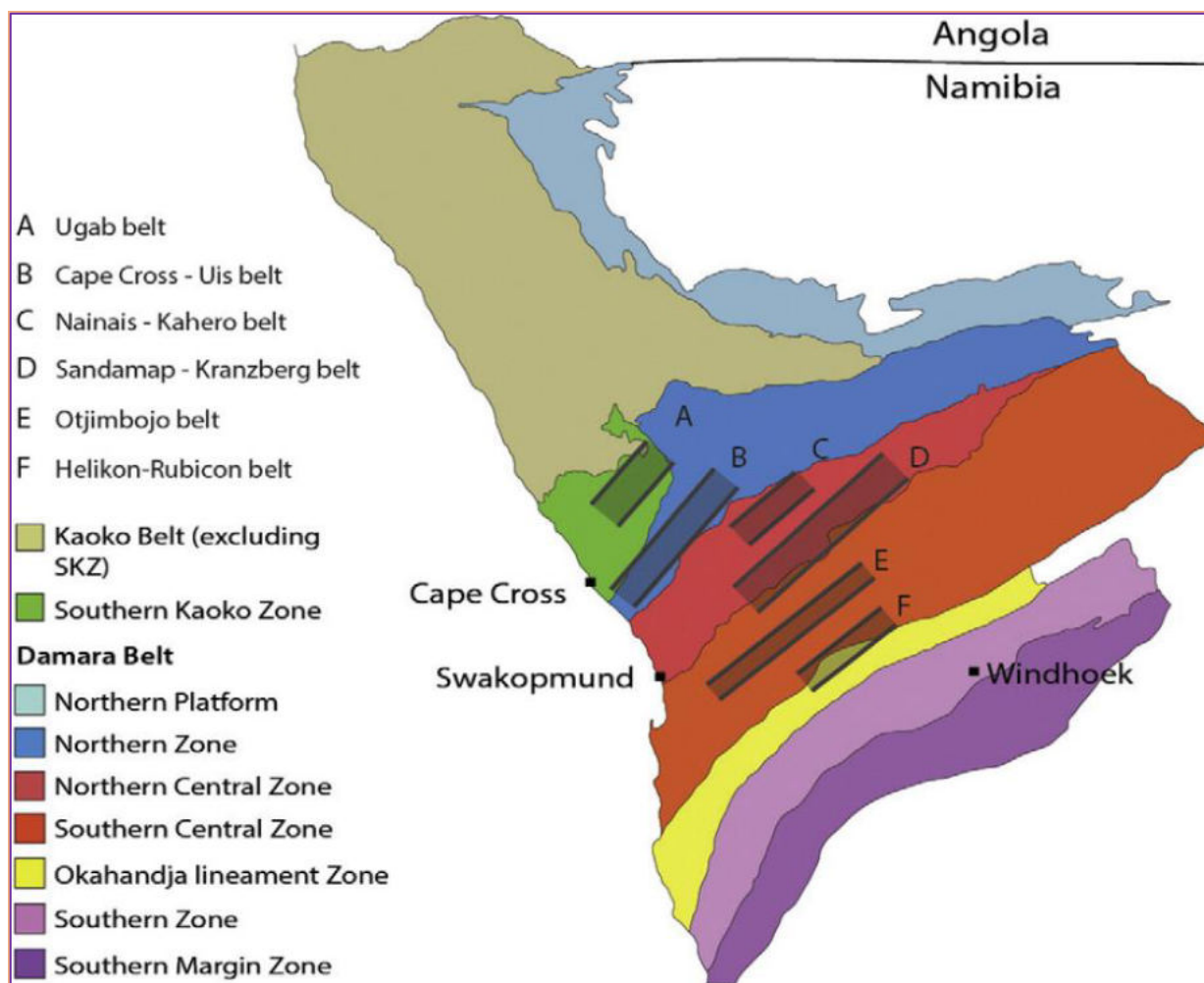
Figure 9: The tectono-stratigraphic zones of the Damara Orogen showing the approximate location of six of the main pegmatite belts (modified after Keller et al., 1999; Miller, 1983; Richards, 1986).
