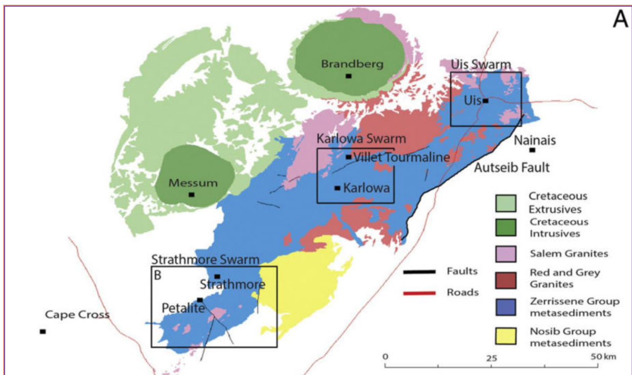
Figure 8: Simplified geological map of the Cape Cross-Uis pegmatite belt, showing metasediments and igneous rocks of the Damara Orogen and post-Damara magmatism
