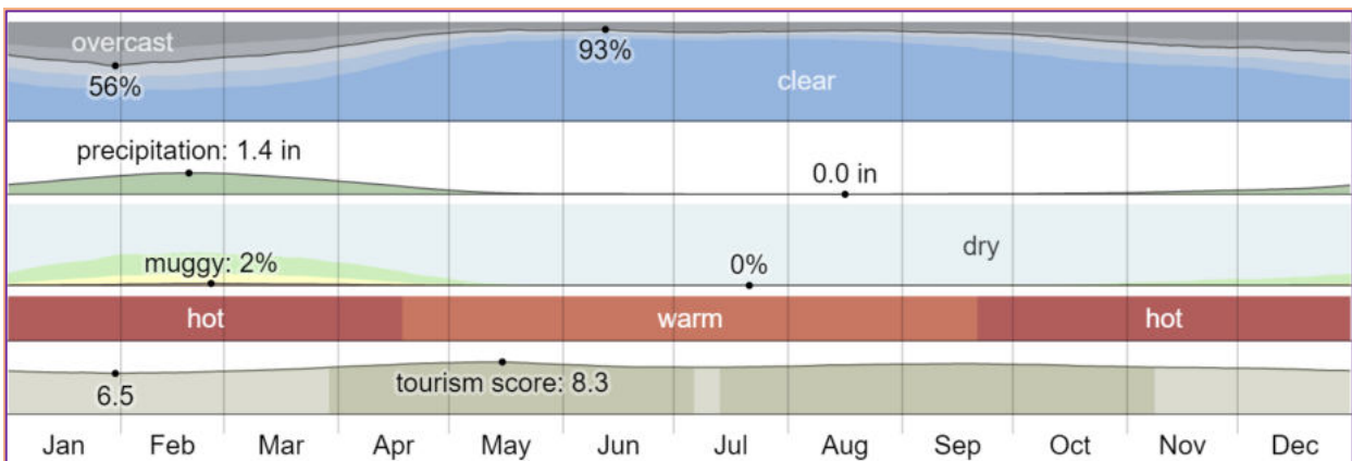
Figure 7: Usakos Climate by month (Weather Sparks, 2022)
