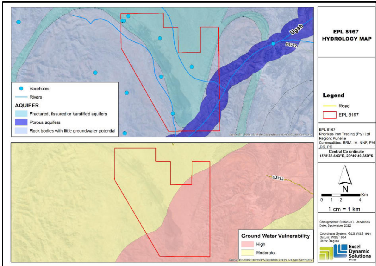
Figure 5: Shows the hydrology map for the EPL
