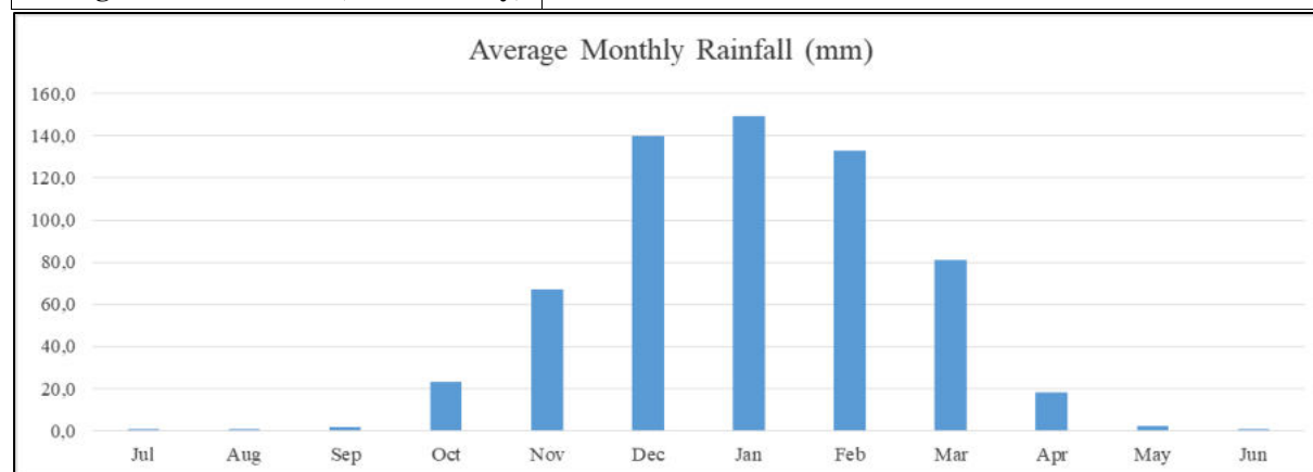
Figure 6-1 Monthly average rainfall (Atlas of Namibia)
