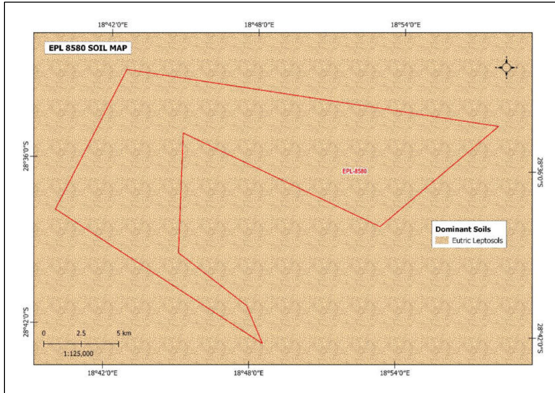
Figure 4: Soil Map showing the dominant soil types found within the EPL area
