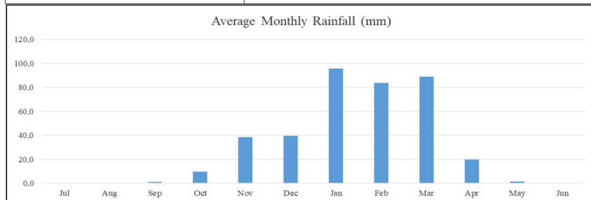
Figure 6-1 Monthly average rainfall (Atlas of Namibia)
