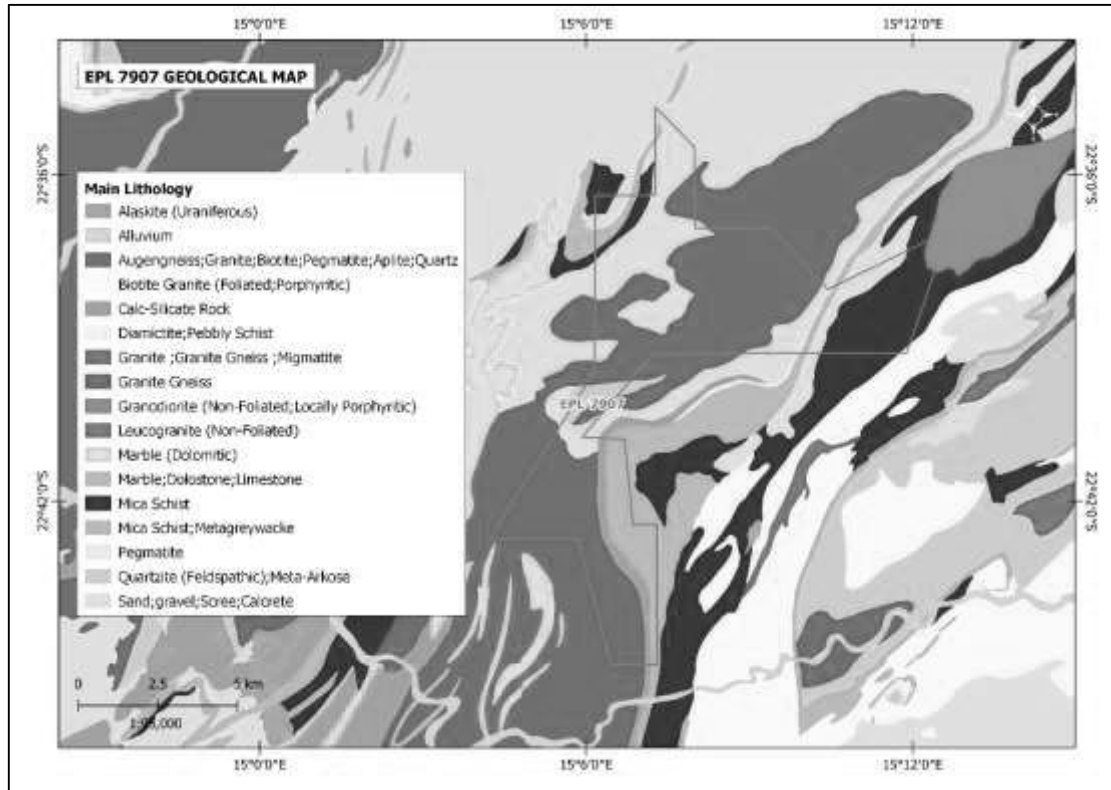
Figure 6: General geology of the project area
