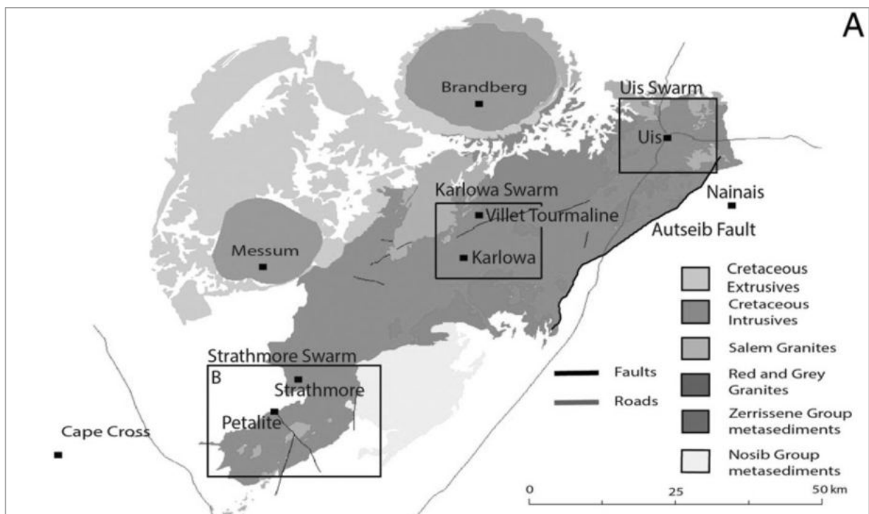
Figure 4: Simplified geological map of the Cape Cross-Uis pegmatite belt, showing metasediments and igneous rocks of the Damara Orogen and post-Damara magmatism
