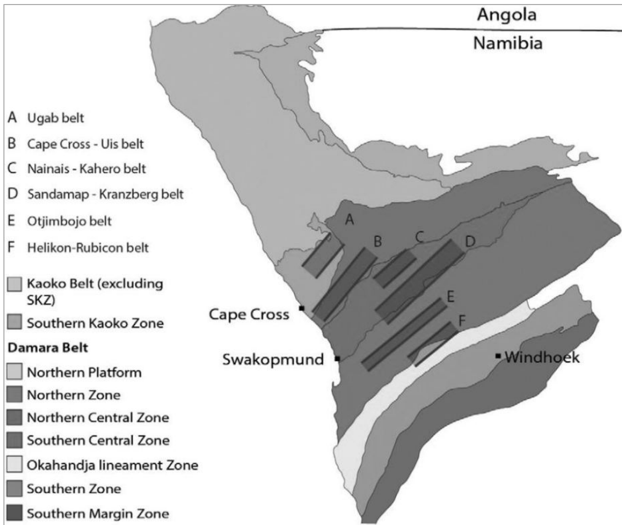
Figure 5: The tectono-stratigraphic zones of the Damara Orogen showing the approximate location of six of the main pegmatite belts (modified after Keller et al., 1999; Miller, 1983; Richards, 1986).
