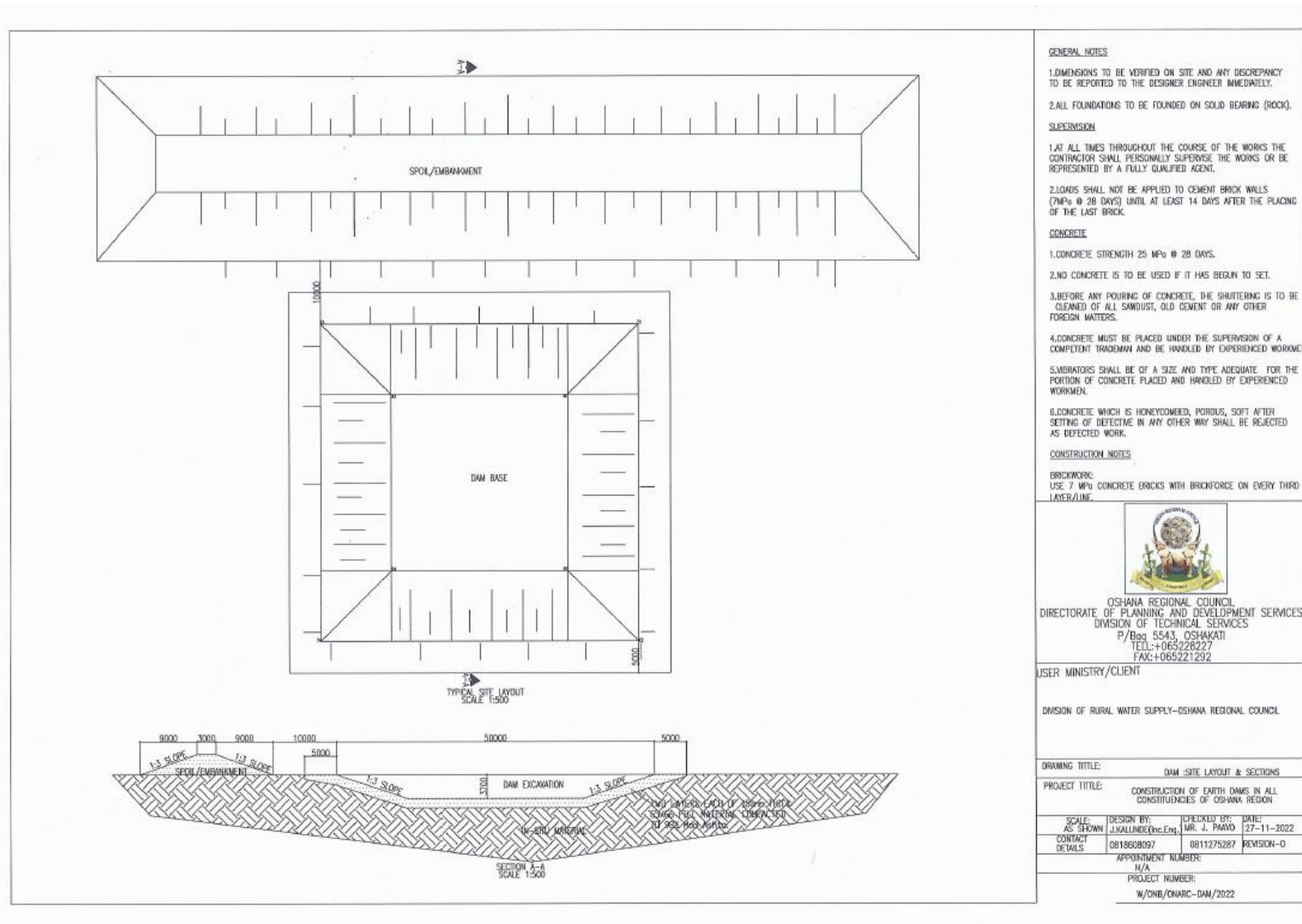
Figure 2-4: Earth Dam Design
