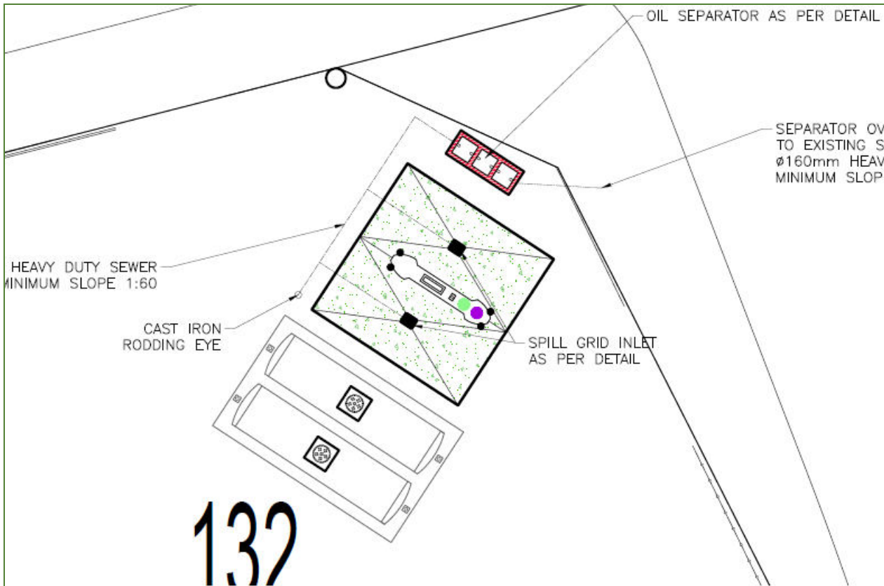
Figure 3. Proposed new site layout plan
