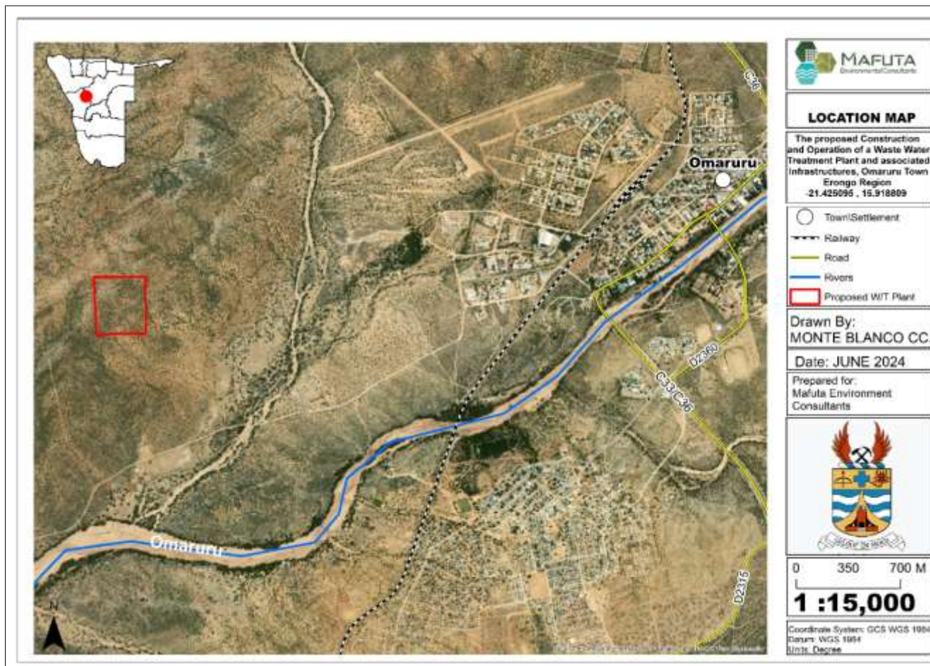
Locality map of the proposed construction and operation of a Wastewater Treatment Plant in Omaruru Town, Erongo Region
