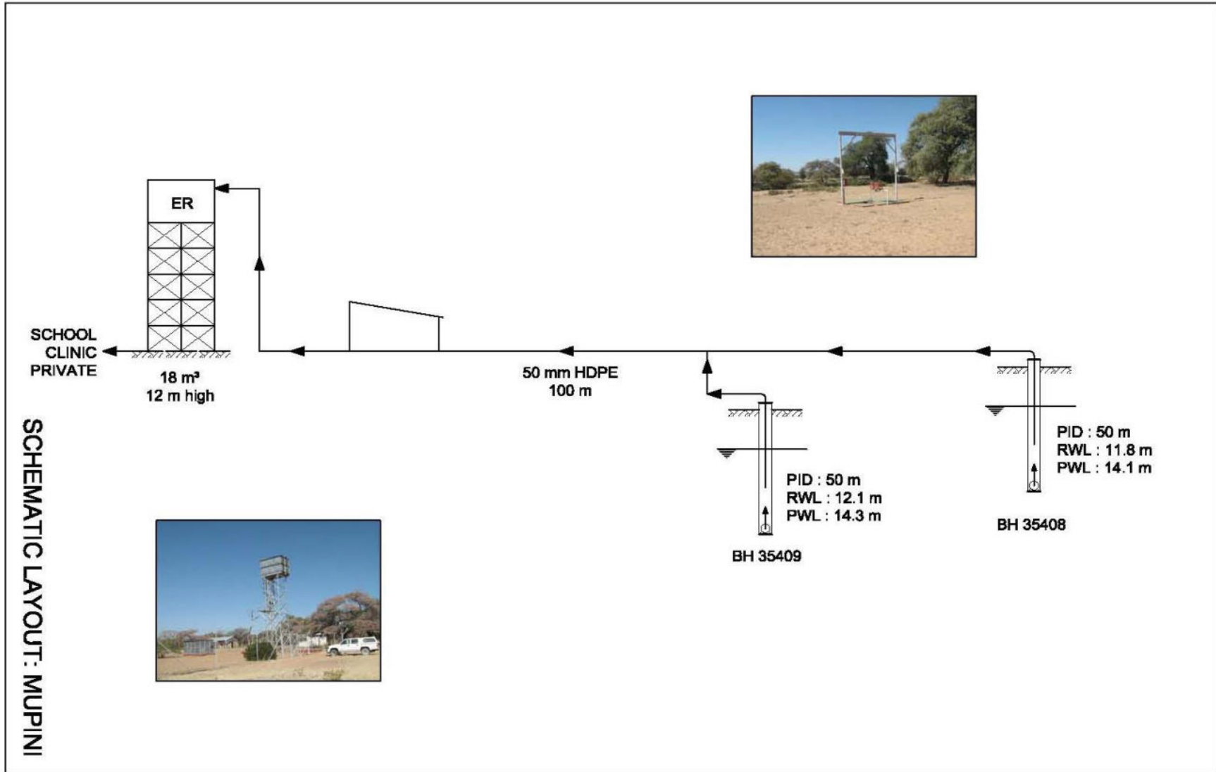
Figure 2: Mupini Scheme Layout
