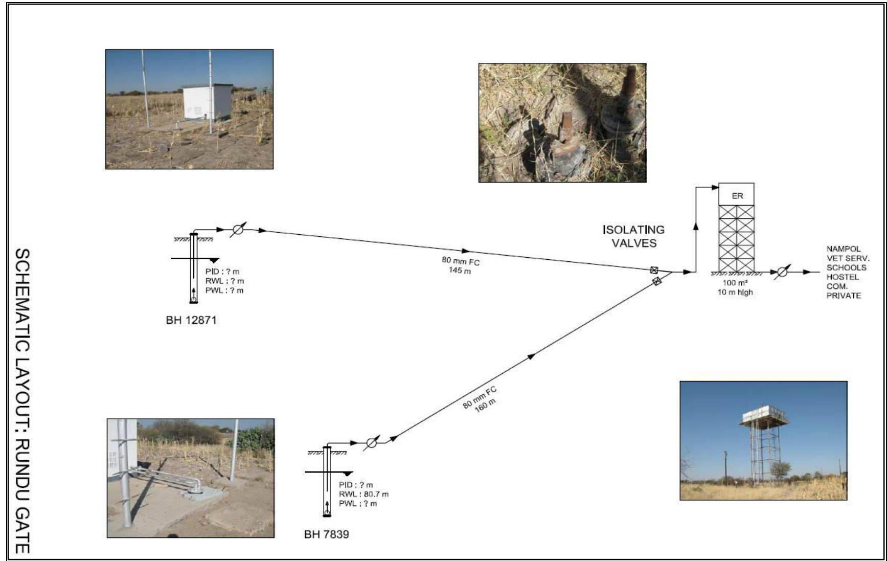
Figure 2: Rundu Gate Scheme Schematic Layout
