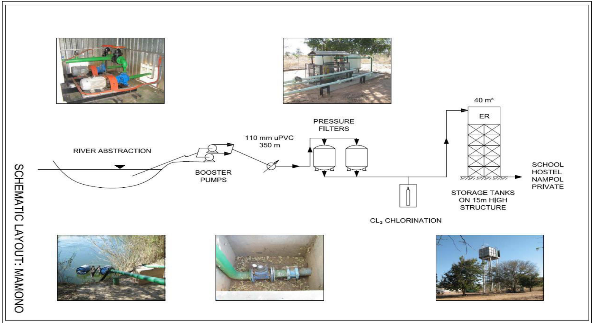
Figure 2: Mamono Scheme Layout
