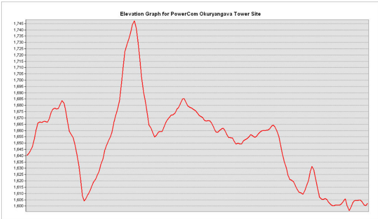
Figure 5 : Elevation graph of the project area
