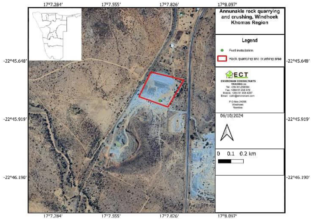
Figure 2: Locality map of Annunakie rock quarrying and crushing
