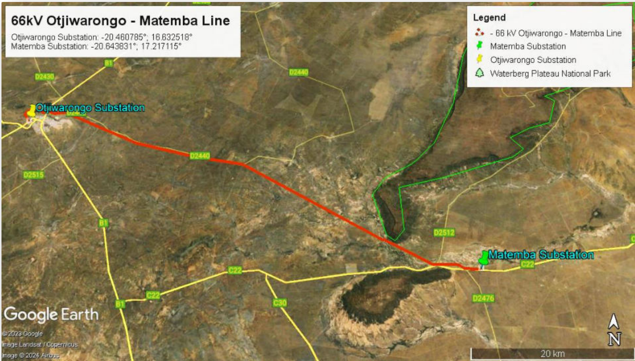
Figure 1: Locality map showing the 66 kV Hardap - Matemba transmission line
