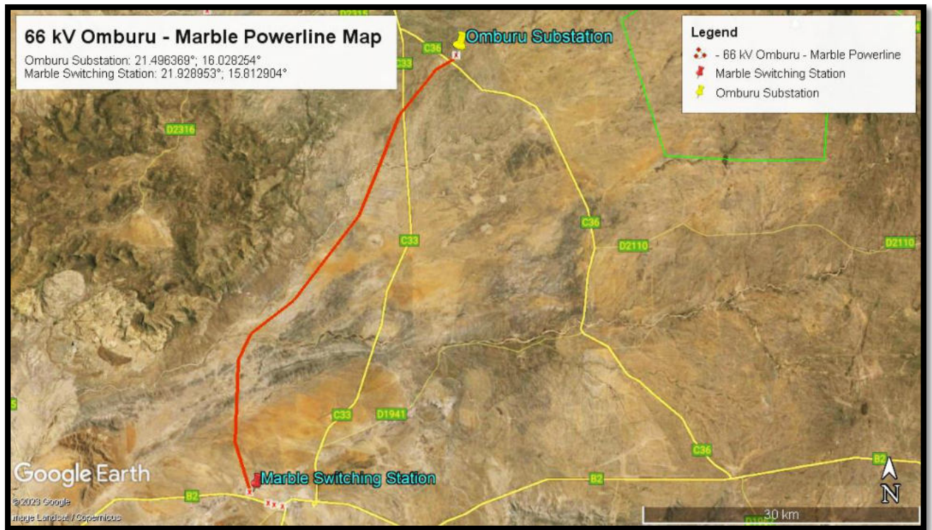
Figure 1: Locality map showing the 66kV Omburu – Marble transmission line
