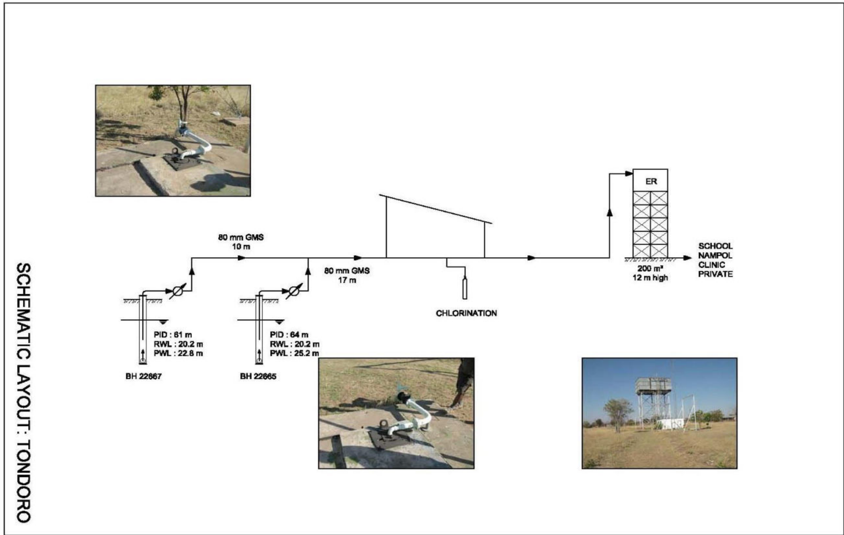
Figure 2: Tondoro Scheme Layout
