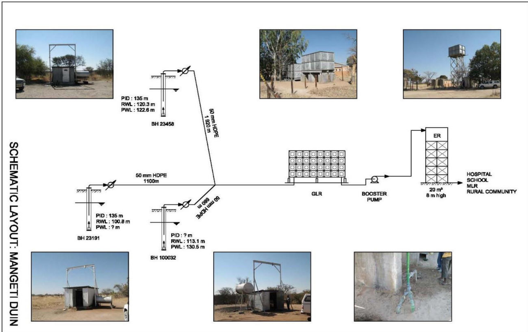
Figure 2: Bukalo Scheme Layout
