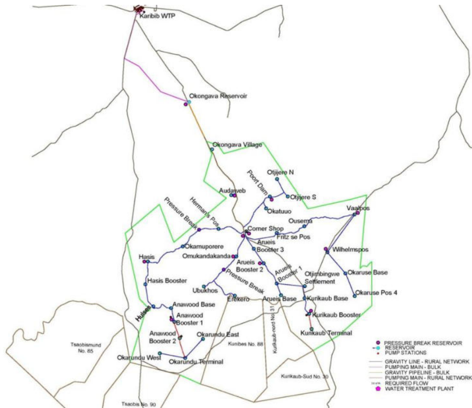
Figure 2: Otjimbingwe Scheme Schematic
