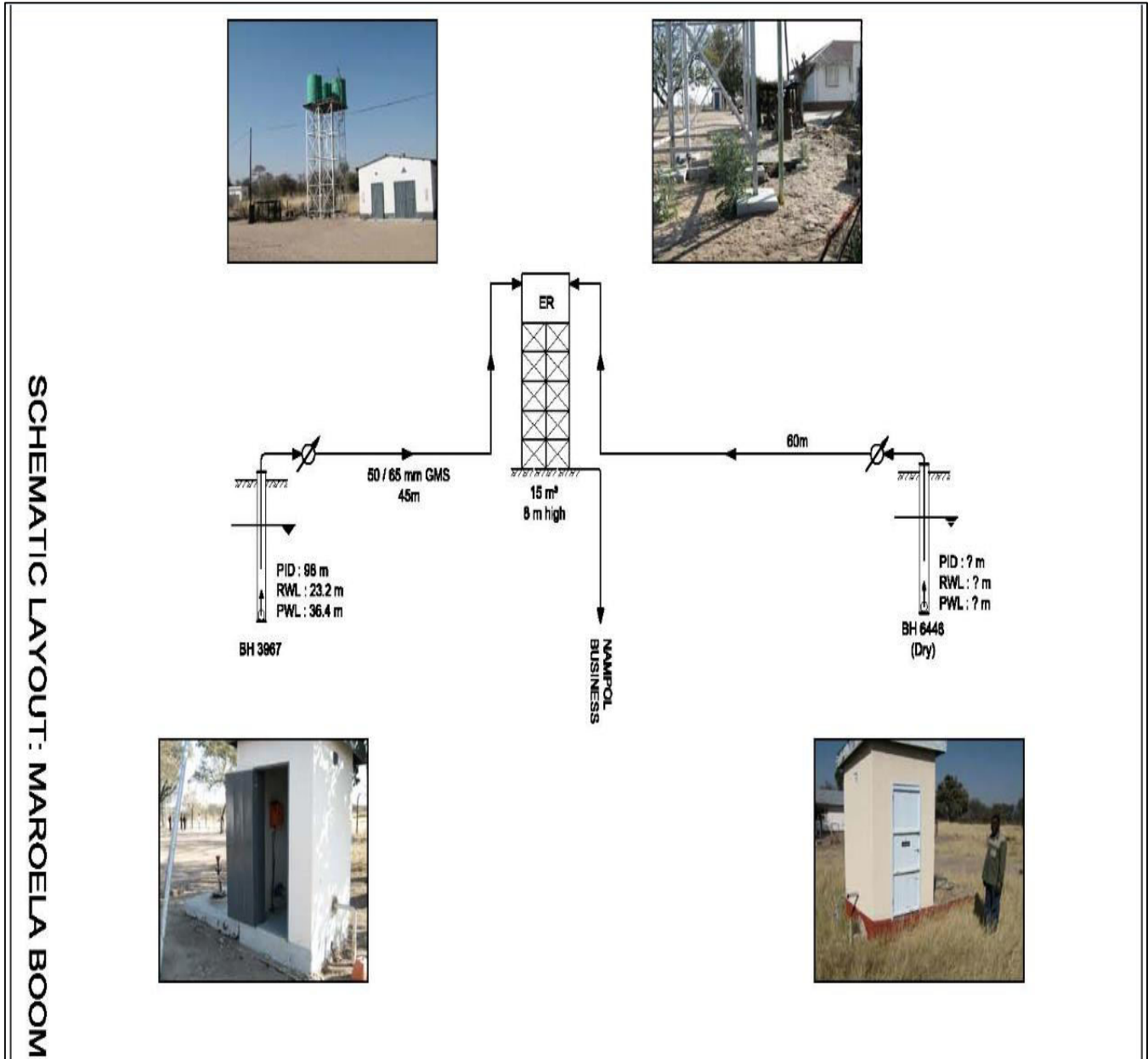
Figure 2: Maroelaboom Scheme Schematic
