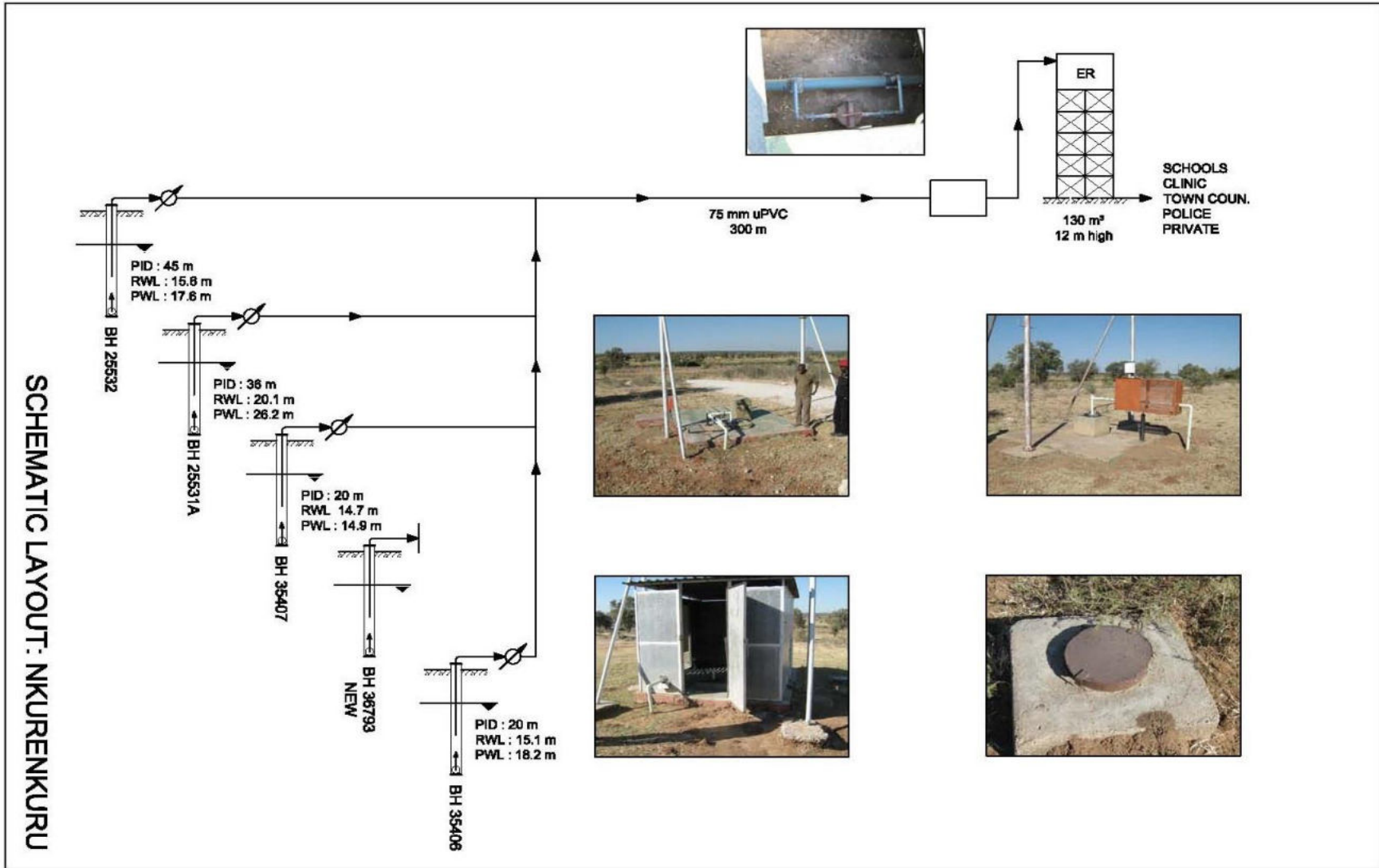
Figure 2: Nkurenkuru Scheme Layout
