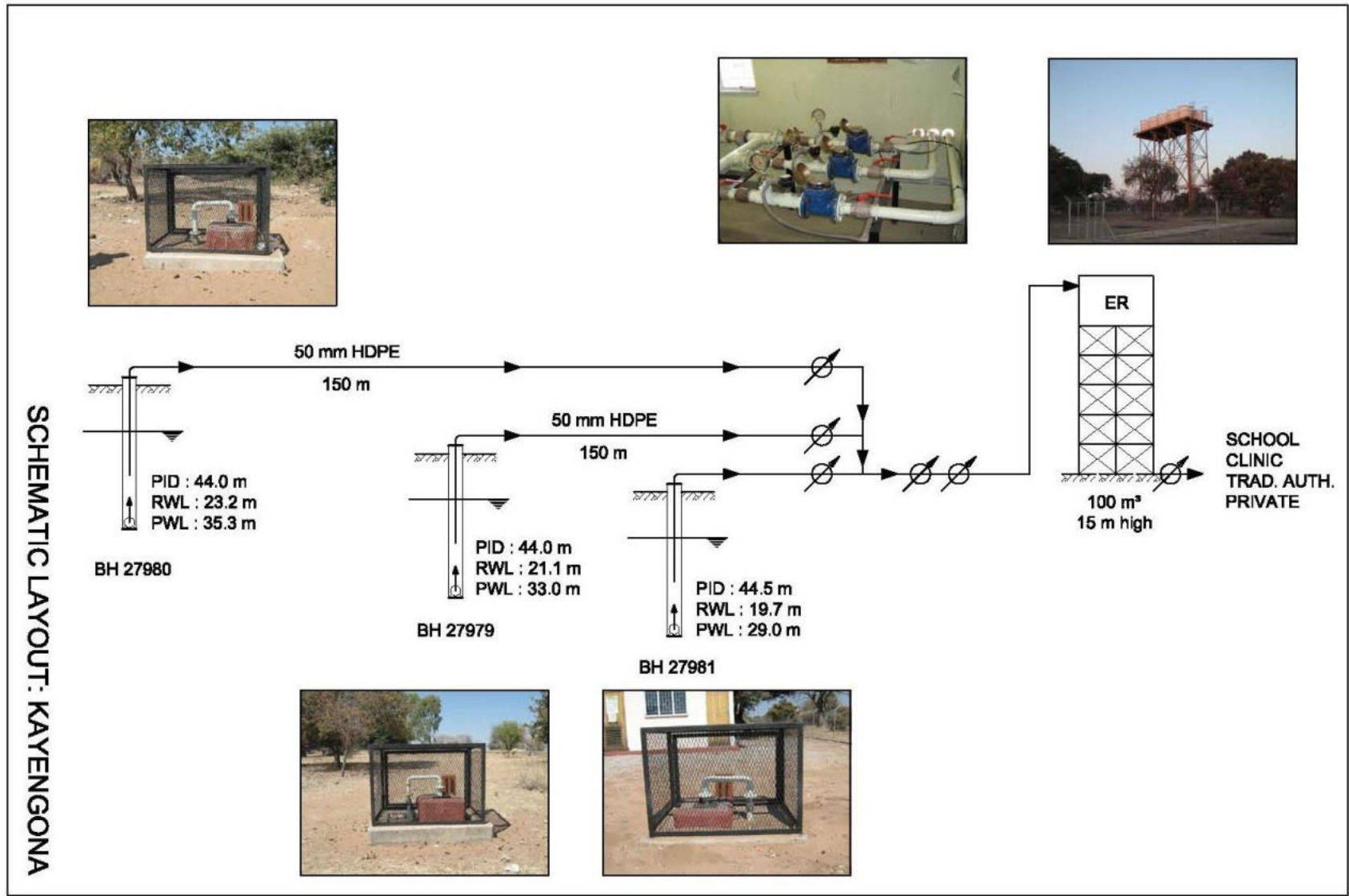
Figure 2: Kayengona Scheme Layout
