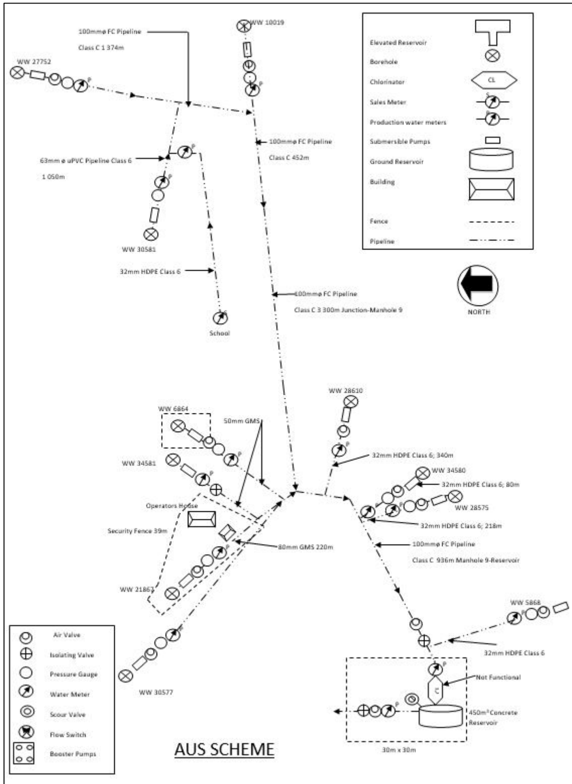
Figure 2: Aus Scheme Layout
