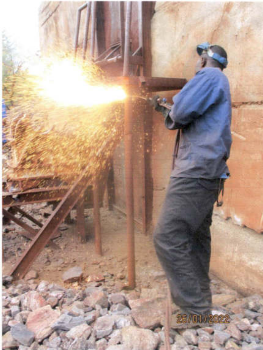
PHOTO 2: The cutting torch operator cutting away the steel supports that carried the disused 10"x21" primary Telsmith Jaw Crusher. The crusher was wrecked and beyond repair. All such steel framework has now been cut down and removed from site.
