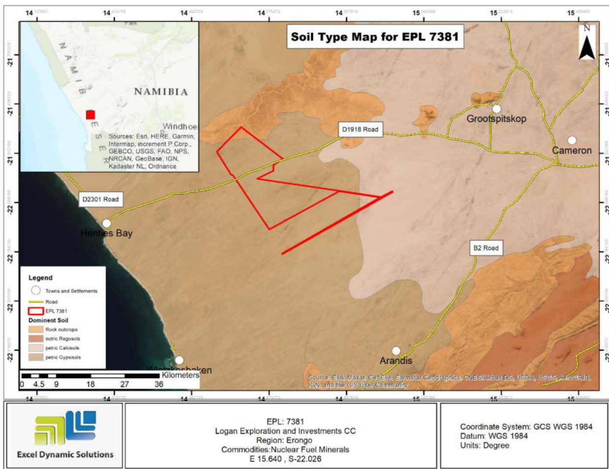
Figure 6: Shows the dominant soil types found within the EPL
