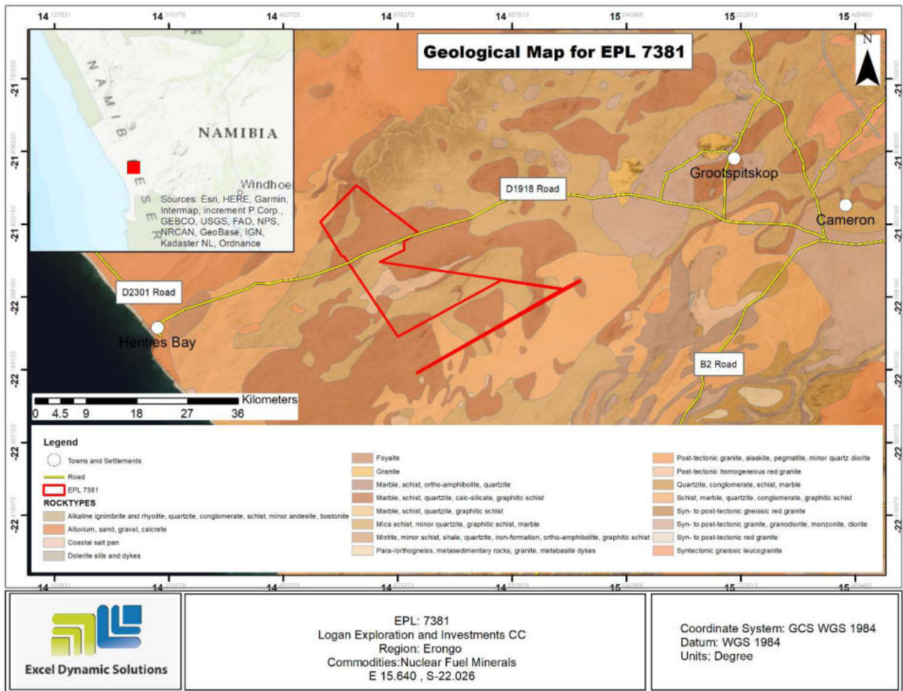
Figure 5: A map of the general geology of the project area
