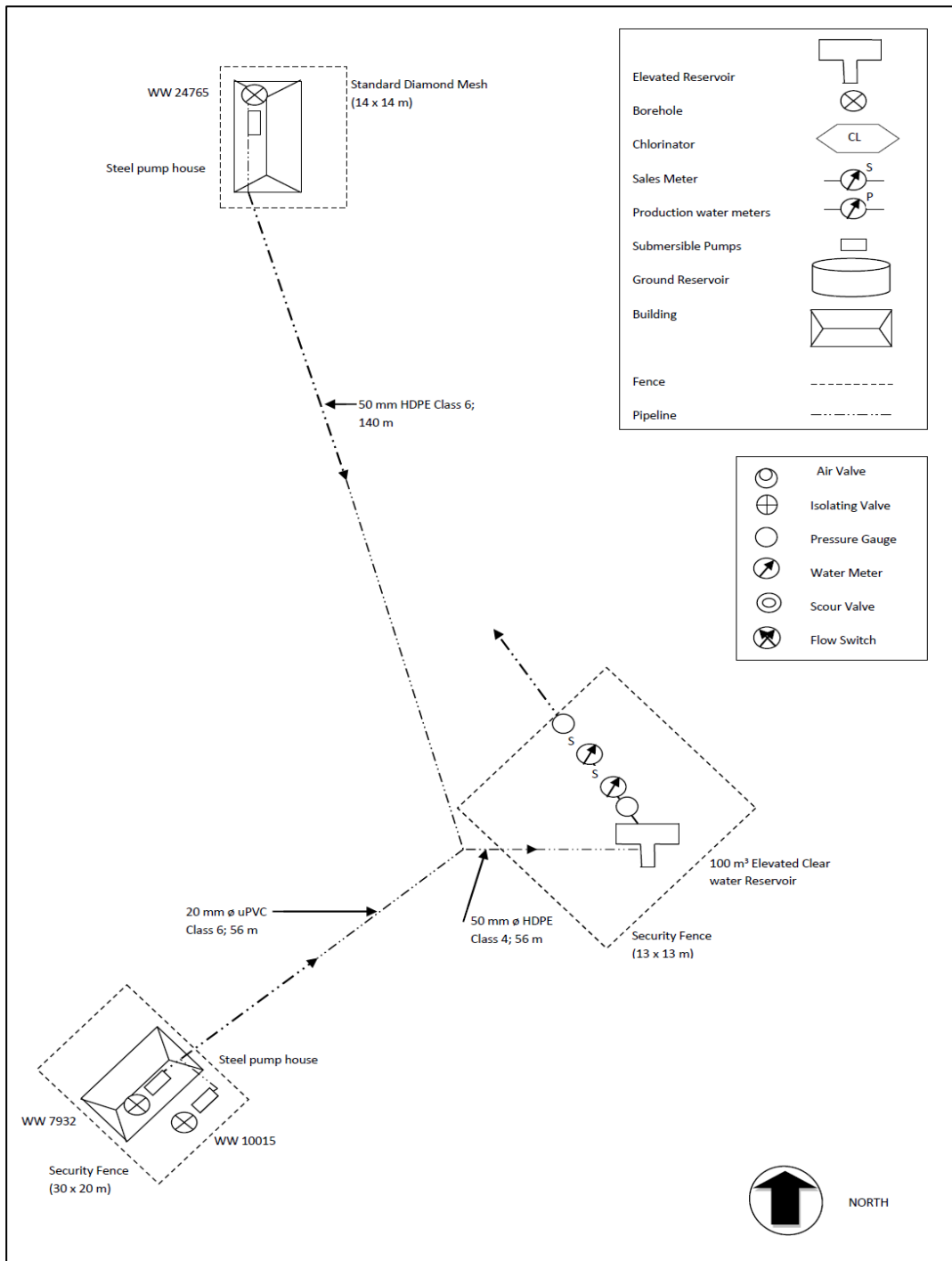
Figure 2: Gainachas Scheme Schematic Layout
