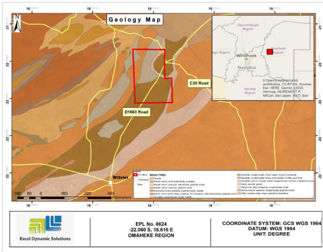
Figure 9: A map of the general geology of the project area
