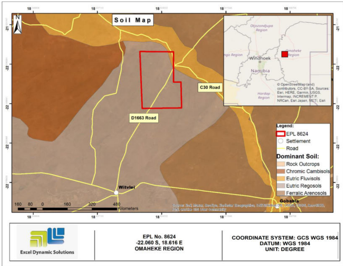
Figure 10: shows the dominant soil types found within the EPL
