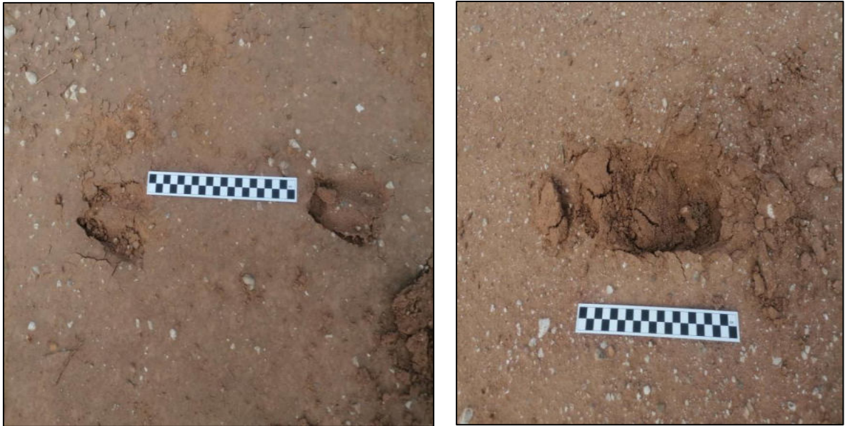
Figure 16: Animal tracks observed during the site visit on 20 April 2022
