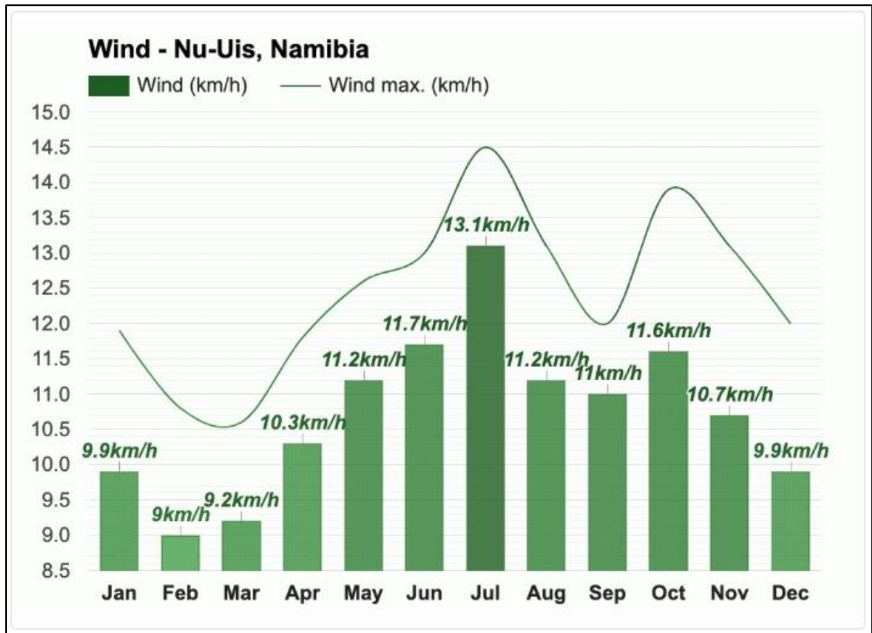
Fig. 20. Wind graph for Nu-Uis and surrounding areas showing maximum and average wind (weather-atlas, 2022).
