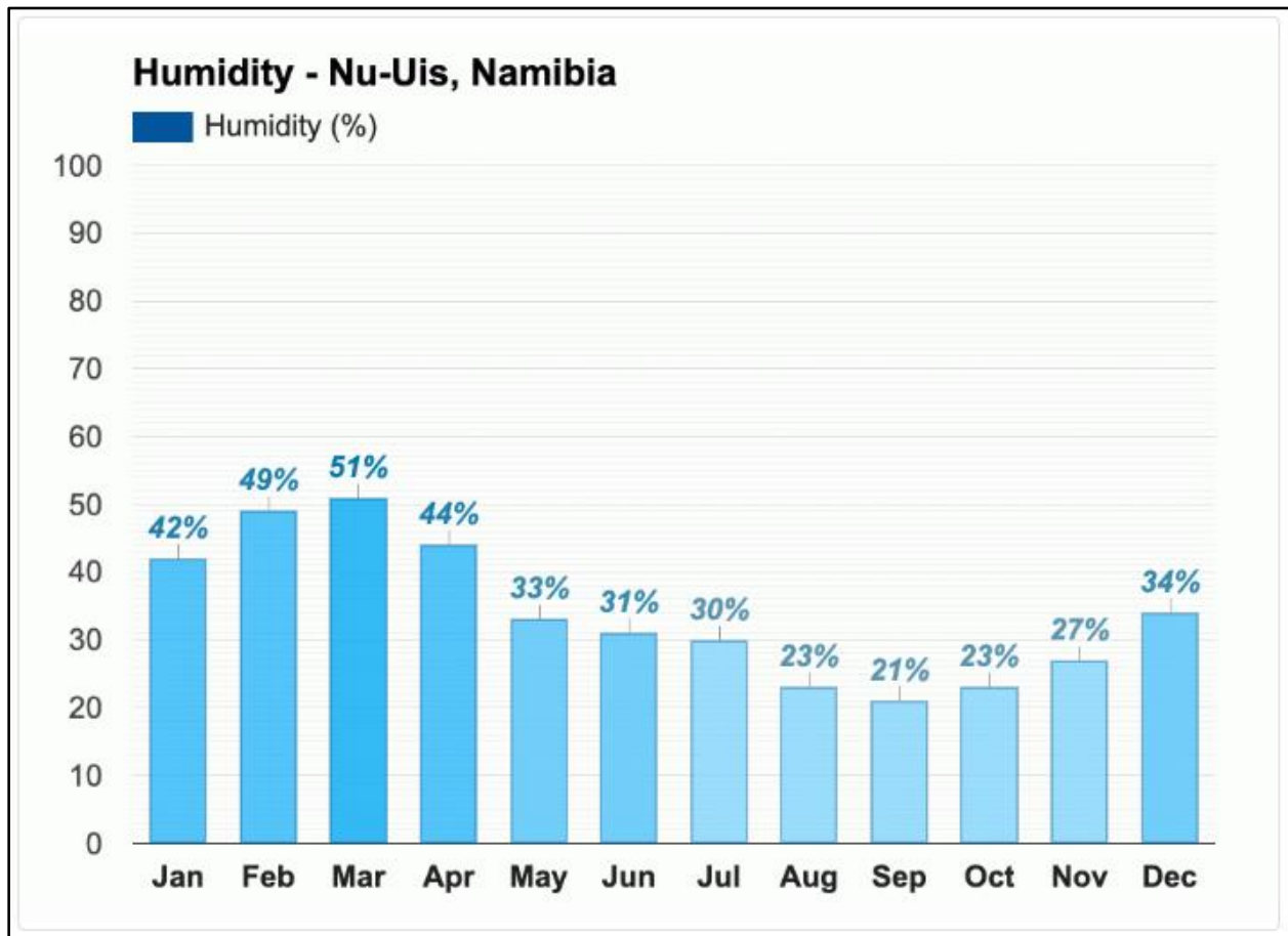
Fig. 21. Humidity graph for Nu-Uis and surrounding areas showing average monthly humidity percentages (weather-atlas, 2022).
