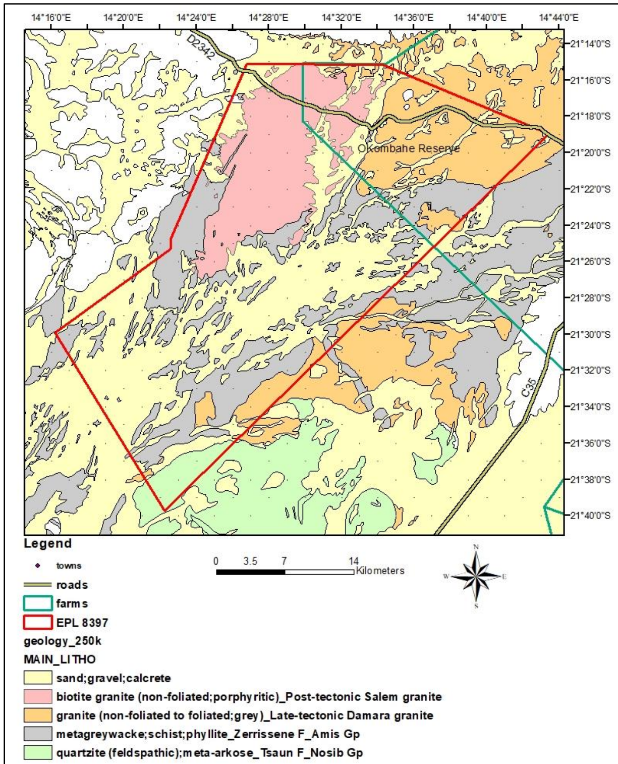
Fig. 24. Detailed local geology of the EPL area.
