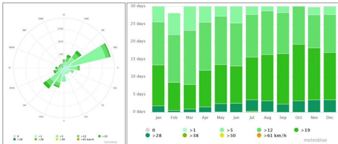
Figure 5-7: A wind rose and wind speed chart for the Wilhelmstal area (Meteoblue, 2023)
