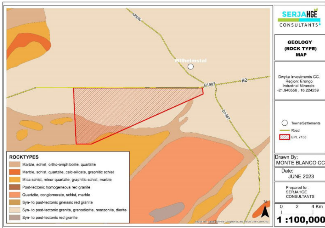
Figure 5-10: The geology of the EPL area
