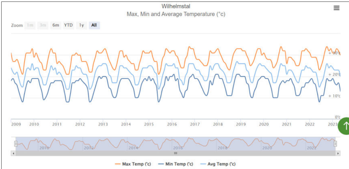
Figure 5-3: The annual maximum, minimum and average temperatures for the Wilhelmstal area (World Weather Online, 2023)
