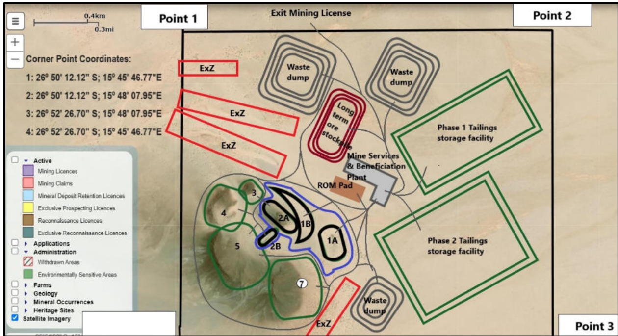
Figure 1: Proposed mine layout plan
