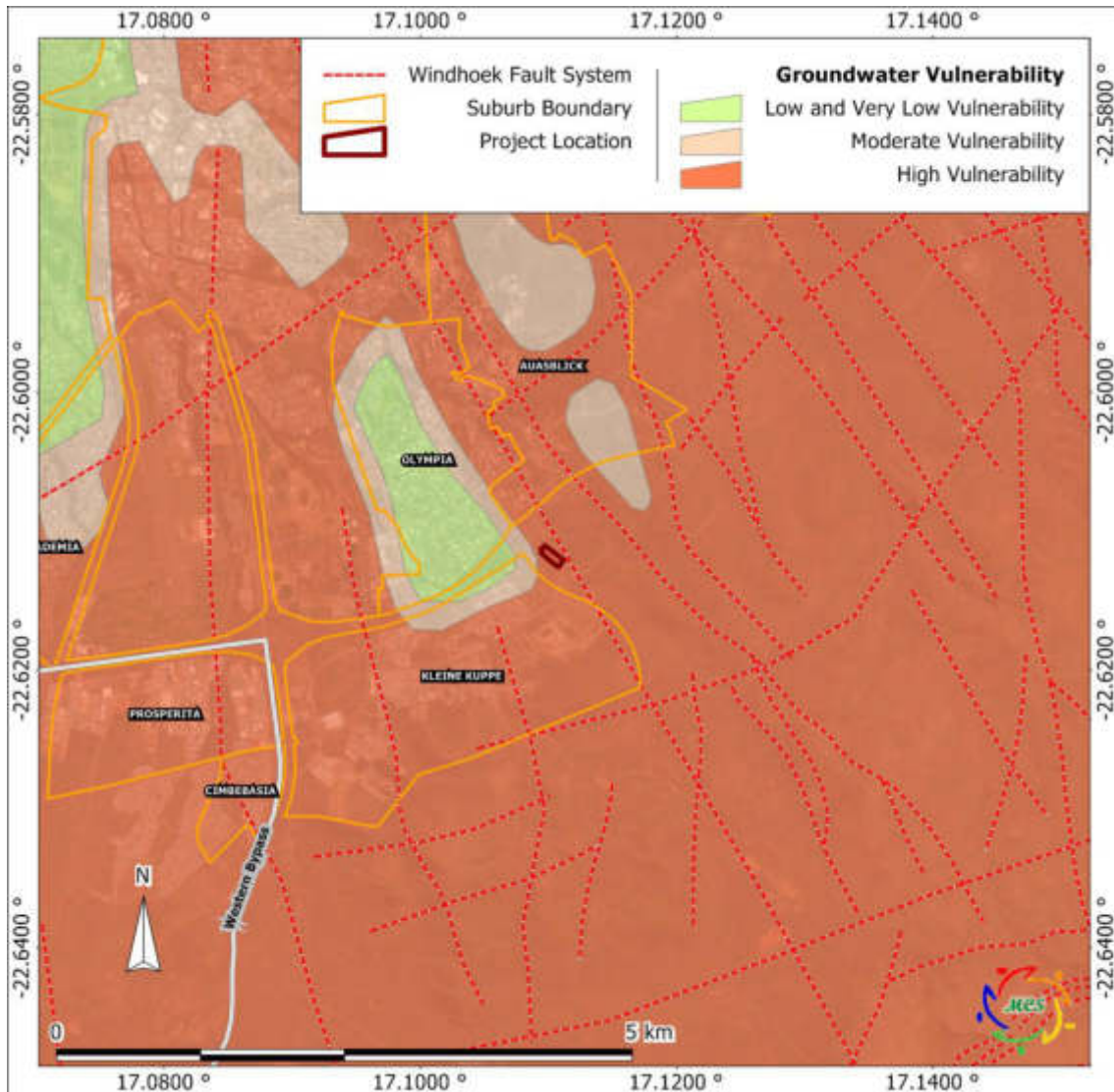
Figure 3. Groundwater Vulnerability Map
