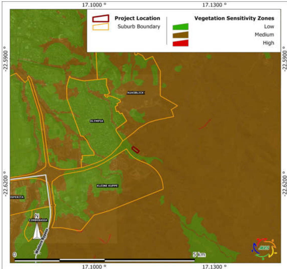
Figure 4. Vegetation Sensitivity of the Project Area
