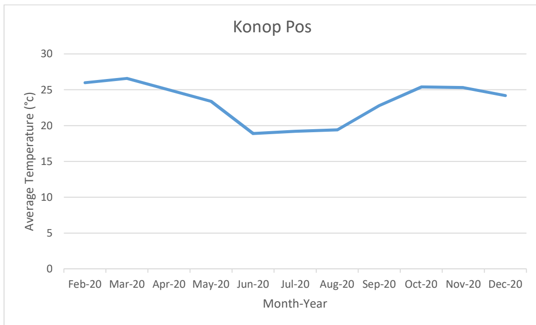
Figure 6: The monthly average temperatures for EPL 8189
