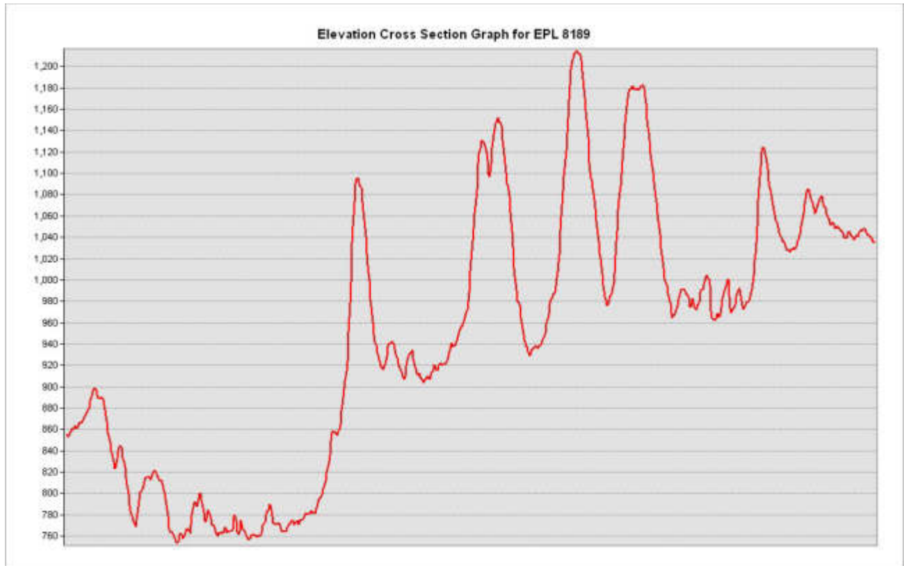
Figure 9 (c): The elevation cross section graph of the project area
