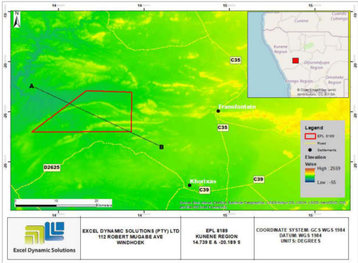
Figure 9 (b): The elevation 3D model map of EPL 8189
