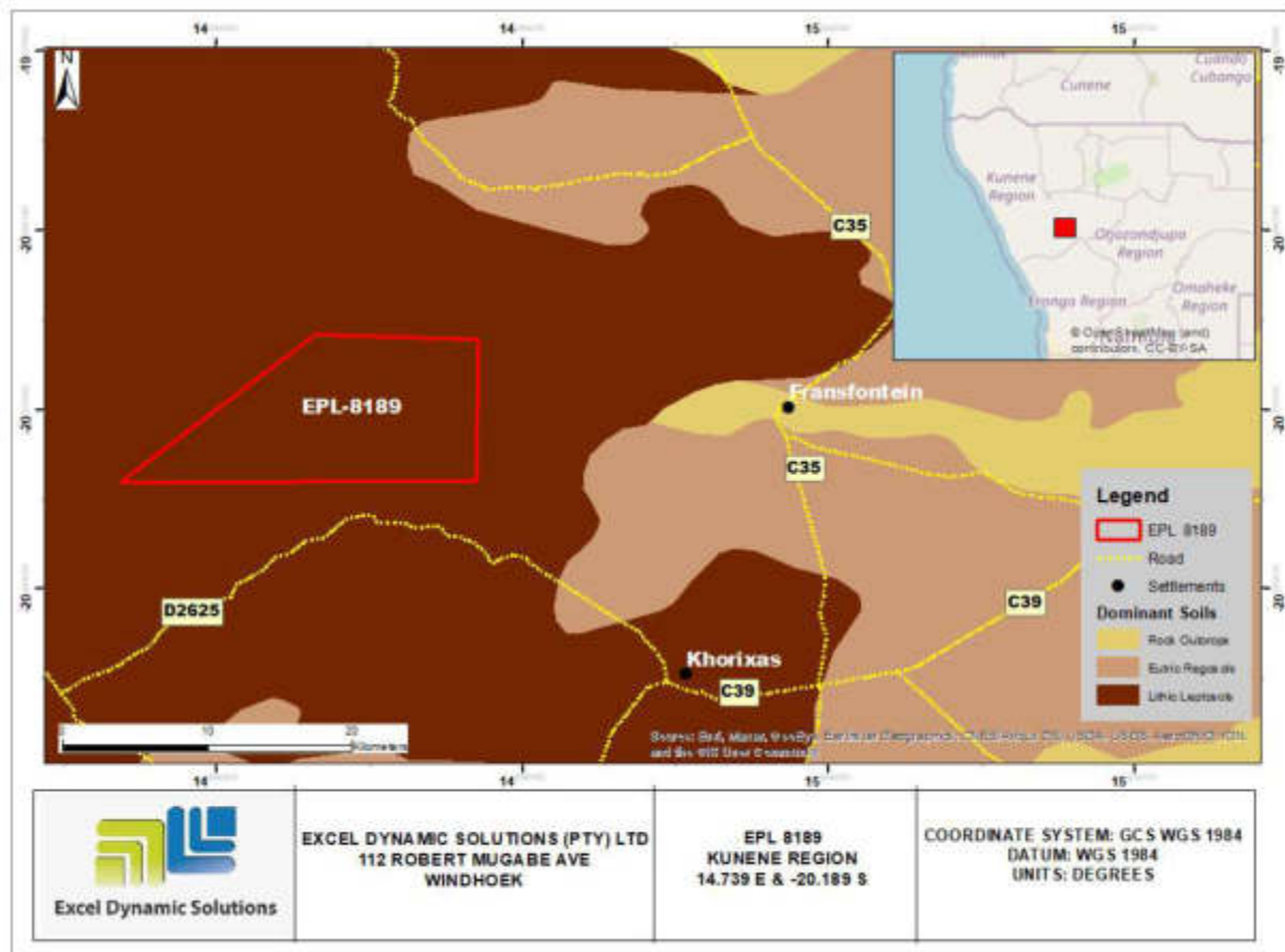
Figure 12: Dominant soil types found within the EPL
