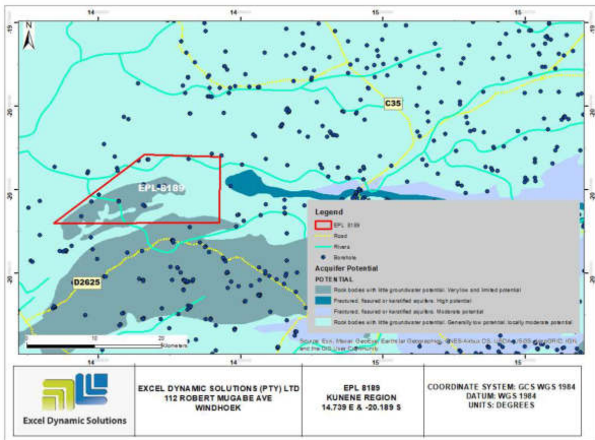
Figure 13: The hydrology and groundwater of the project area
