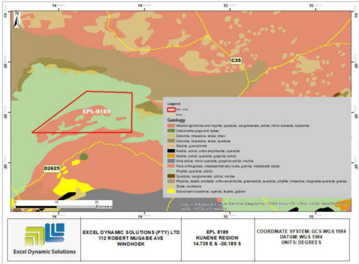
Figure 10: The geology of the EPL and surrounding project area
