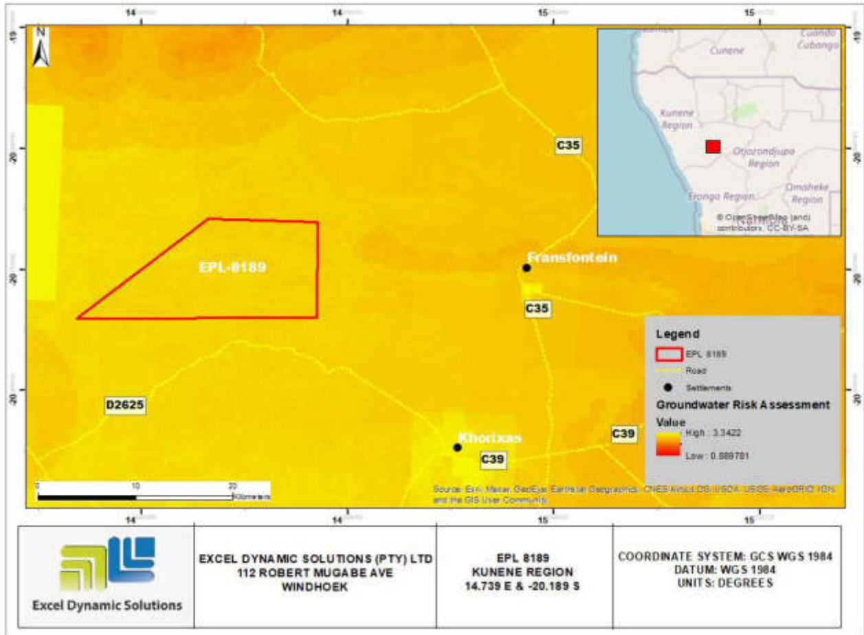
Figure 14: Groundwater Drought Risk map around the project area
