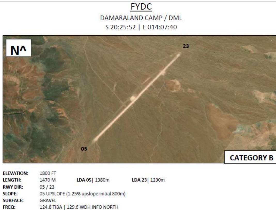
Figure 5: The Damaraland Camp airstrip
