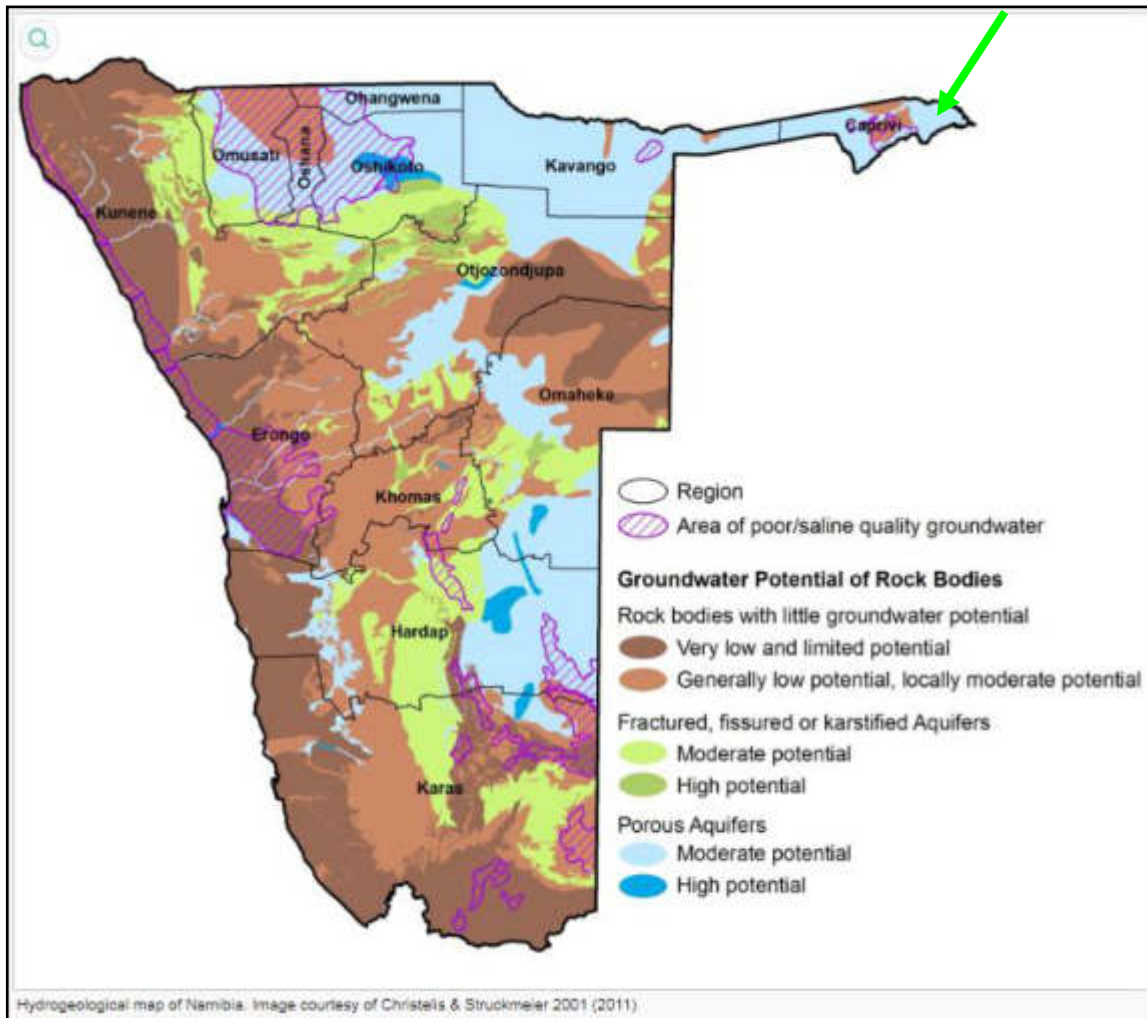
Figure 4: Hydrogeological map of Namibia with rock bodies groundwater potential with the approximate location of Mpukano site in far eastern Namibia (green arrow)
