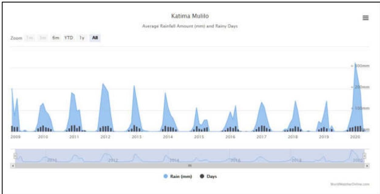
Figure 2: The rainfall patterns for the Katima Mulilo area (source: World Weather Online, 2020)
