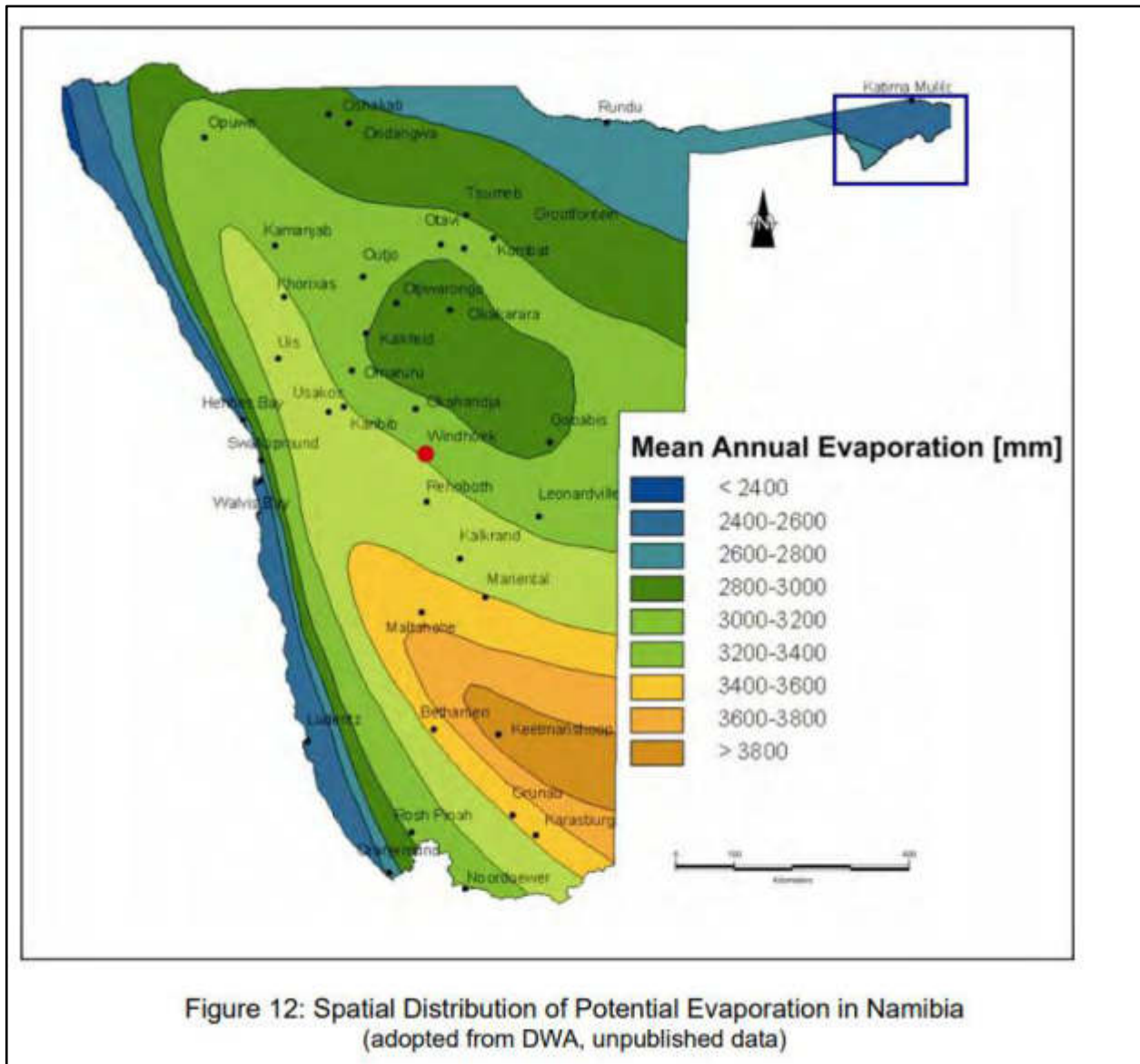
Figure 1: The spatial distribution of potential evaporation in Namibia (after BGR, 2005)
