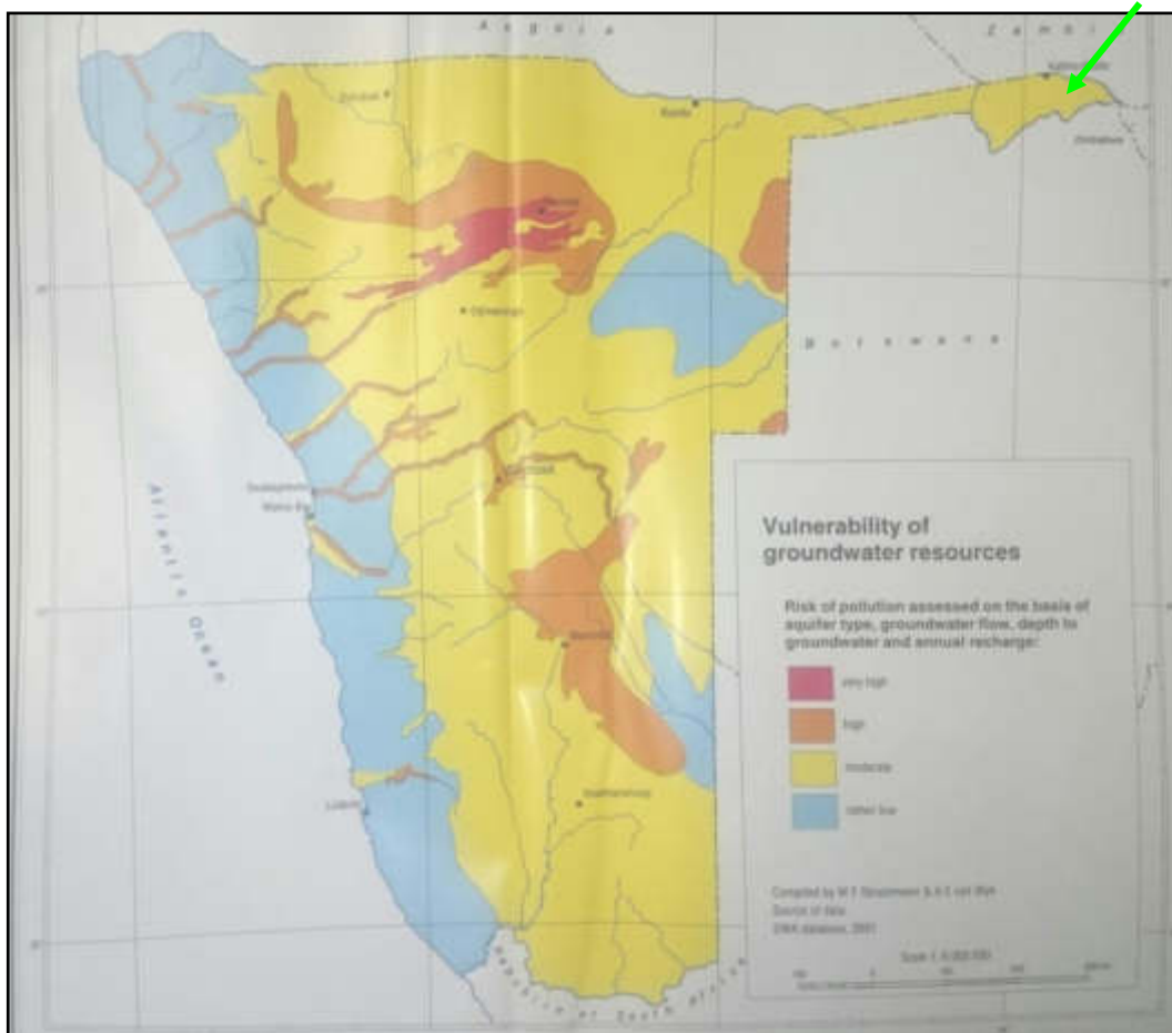
Figure 5: Vulnerability of groundwater resources to Pollution (Van Wyk et.al, 2001)- project site area shown by the green arrow)
