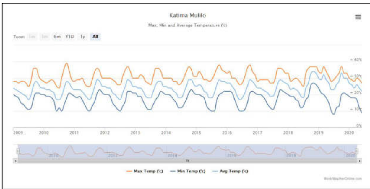
Figure 3: The maximum, minimum and average temperature Katima Mulilo area (source: World Weather Online, 2020)
